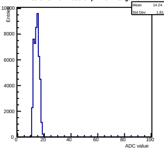
Ped ch 8 mcm 2000 chip 4 nominal-gain0
