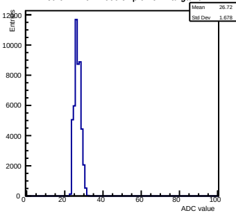
Ped ch 1 mcm 2000 chip 0 nominal-gain0
