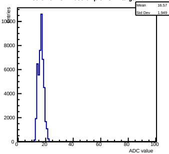
Ped ch 0 mcm 2000 chip 0 nominal-gain0
