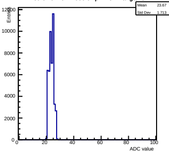
Ped ch 9 mcm 2000 chip 4 nominal-gain0
