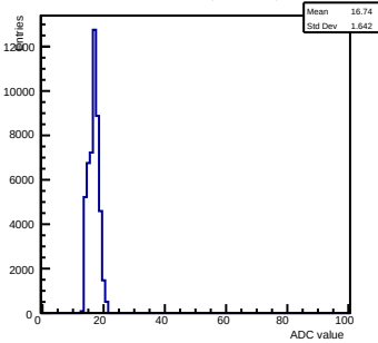
Ped ch 15 mcm 2000 chip 7 nominal-gain0
