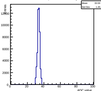
Pedestals ch 4 chip 2003 nominal-gain0
