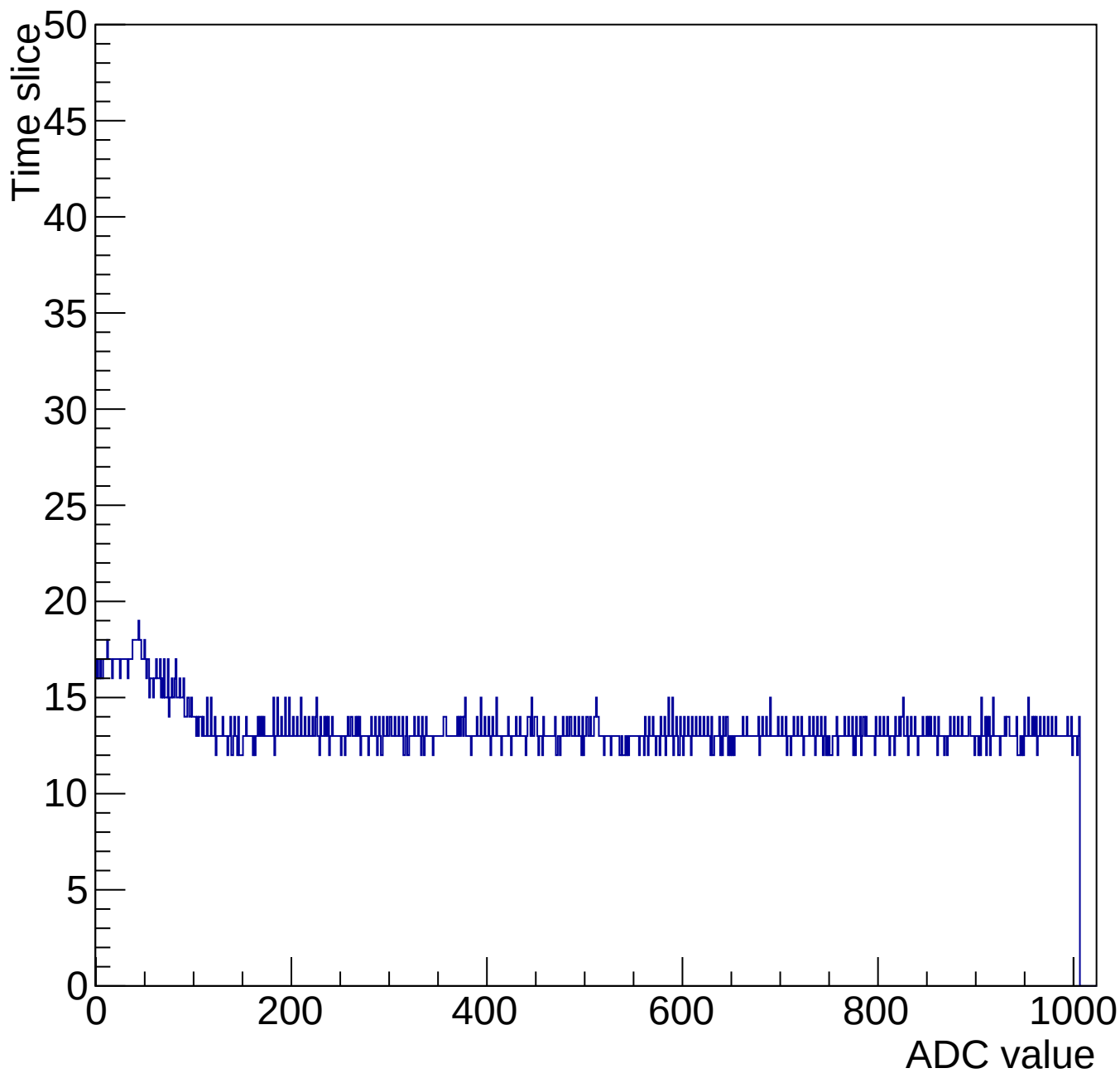
Evt 10 Time ch 3 chip 2003 preamp0gain0shaper0decay0.5
