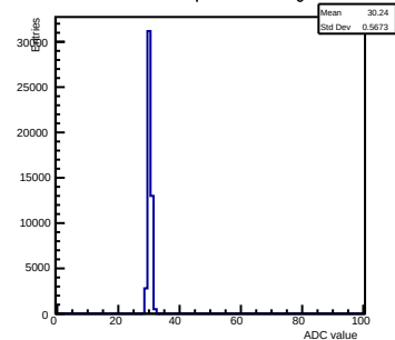
Pedestals ch 4 chip 2002 nominal-gain0
