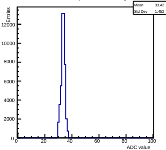
Pedestals ch 4 chip 2003 nominal-gain0
