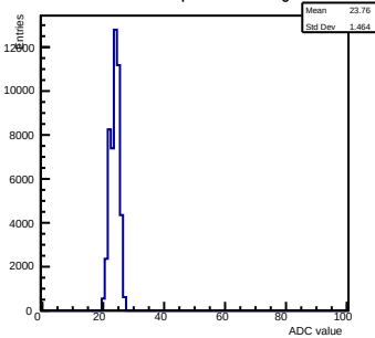
Pedestals ch 9 chip 2003 nominal-gain0
