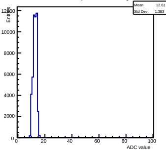
Pedestals ch 12 chip 2003 nominal-gain0
