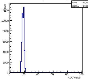
Pedestals ch 6 chip 2003 nominal-gain0
