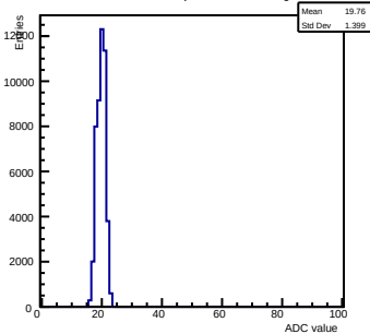
Pedestals ch 13 chip 2003 nominal-gain0
