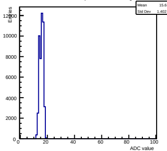
Pedestals ch 15 chip 2003 nominal-gain0
