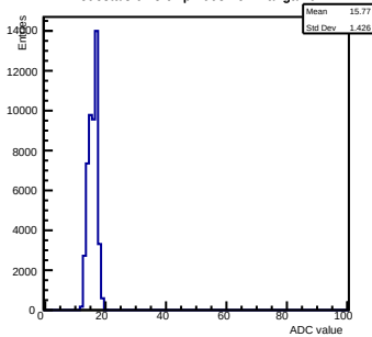
Pedestals ch 3 chip 2003 nominal-gain0
