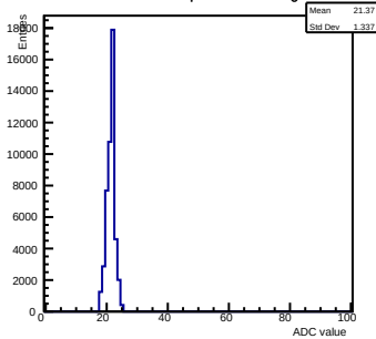
Pedestals ch 11 chip 2003 nominal-gain0
