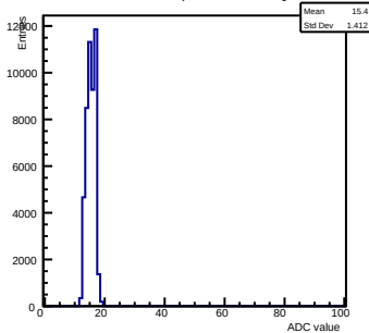
Pedestals ch 7 chip 2003 nominal-gain0
