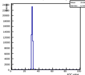
Pedestals ch 7 chip 2004 nominal-gain0
