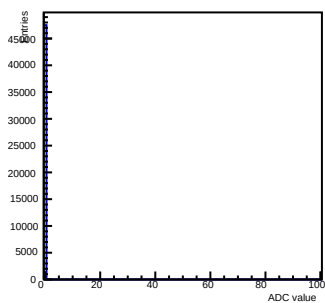
Pedestals ch 3 chip 2004 nominal-gain0
