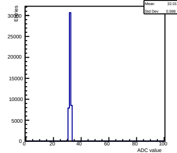
Pedestals ch 0 chip 2004 nominal-gain0
