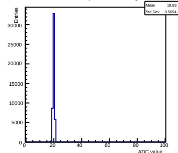
Pedestals ch 4 chip 2004 nominal-gain0
