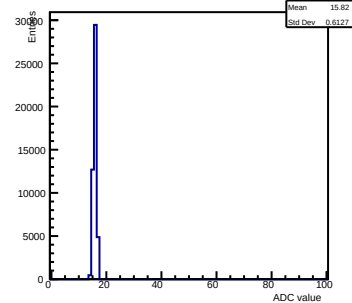
Pedestals ch 8 chip 2004 nominal-gain0
