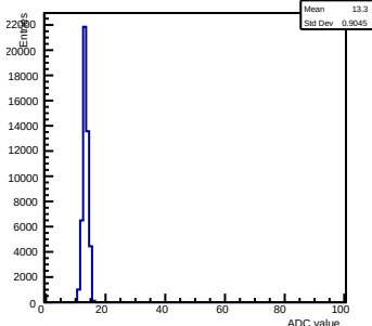
Pedestals ch 13 chip 2005 nominal-gain0
