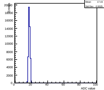
Pedestals ch 11 chip 2005 nominal-gain0
