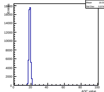
Pedestals ch 14 chip 2005 nominal-gain0
