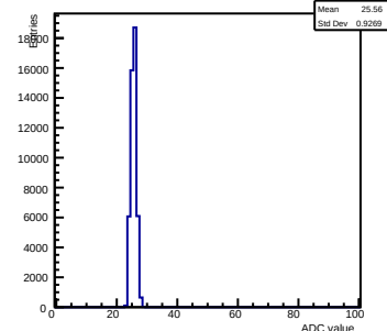
Pedestals ch 7 chip 2005 nominal-gain0
