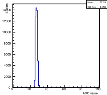
Pedestals ch 1 chip 2005 nominal-gain0
