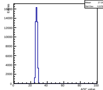
Pedestals ch 6 chip 2005 nominal-gain0
