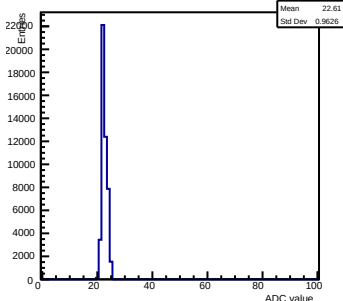
Pedestals ch 5 chip 2005 nominal-gain0
