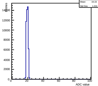
Pedestals ch 9 chip 2005 nominal-gain0
