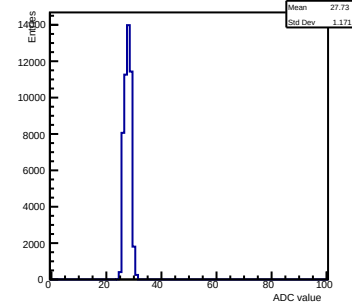
Pedestals ch 0 chip 2005 nominal-gain0
