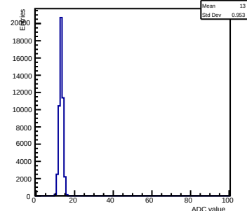
Pedestals ch 4 chip 2005 nominal-gain0
