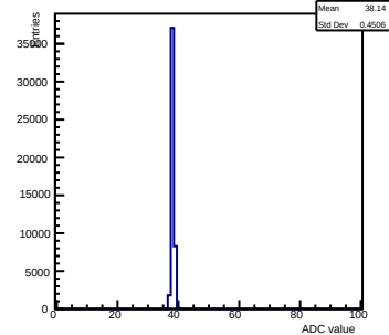
Pedestals ch 0 chip 2006 nominal-gain0
