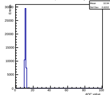
Pedestals ch 4 chip 2006 nominal-gain0
