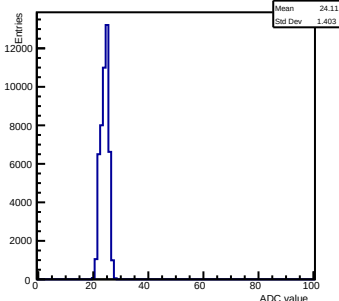
Pedestals ch 6 chip 2007 nominal-gain0
