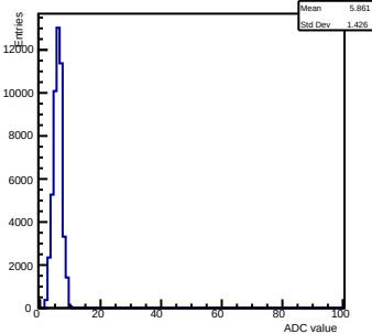
Pedestals ch 0 chip 2007 nominal-gain0
