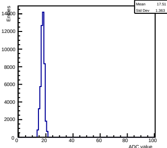
Pedestals ch 15 chip 2007 nominal-gain0
