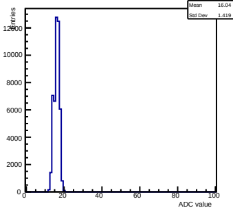
Pedestals ch 2 chip 2007 nominal-gain0
