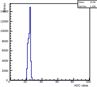
Pedestals ch 1 chip 2007 nominal-gain0
