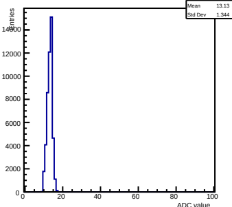
Pedestals ch 12 chip 2007 nominal-gain0
