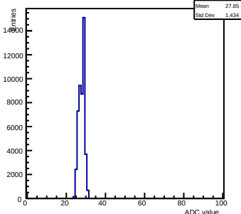
Pedestals ch 14 chip 2007 nominal-gain0
