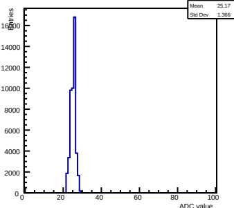
Pedestals ch 13 chip 2007 nominal-gain0
