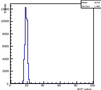
Pedestals ch 4 chip 2007 nominal-gain0
