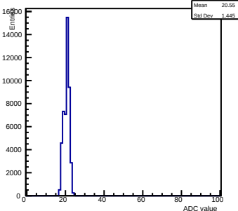
Pedestals ch 11 chip 2007 nominal-gain0
