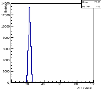
Pedestals ch 10 chip 2007 nominal-gain0
