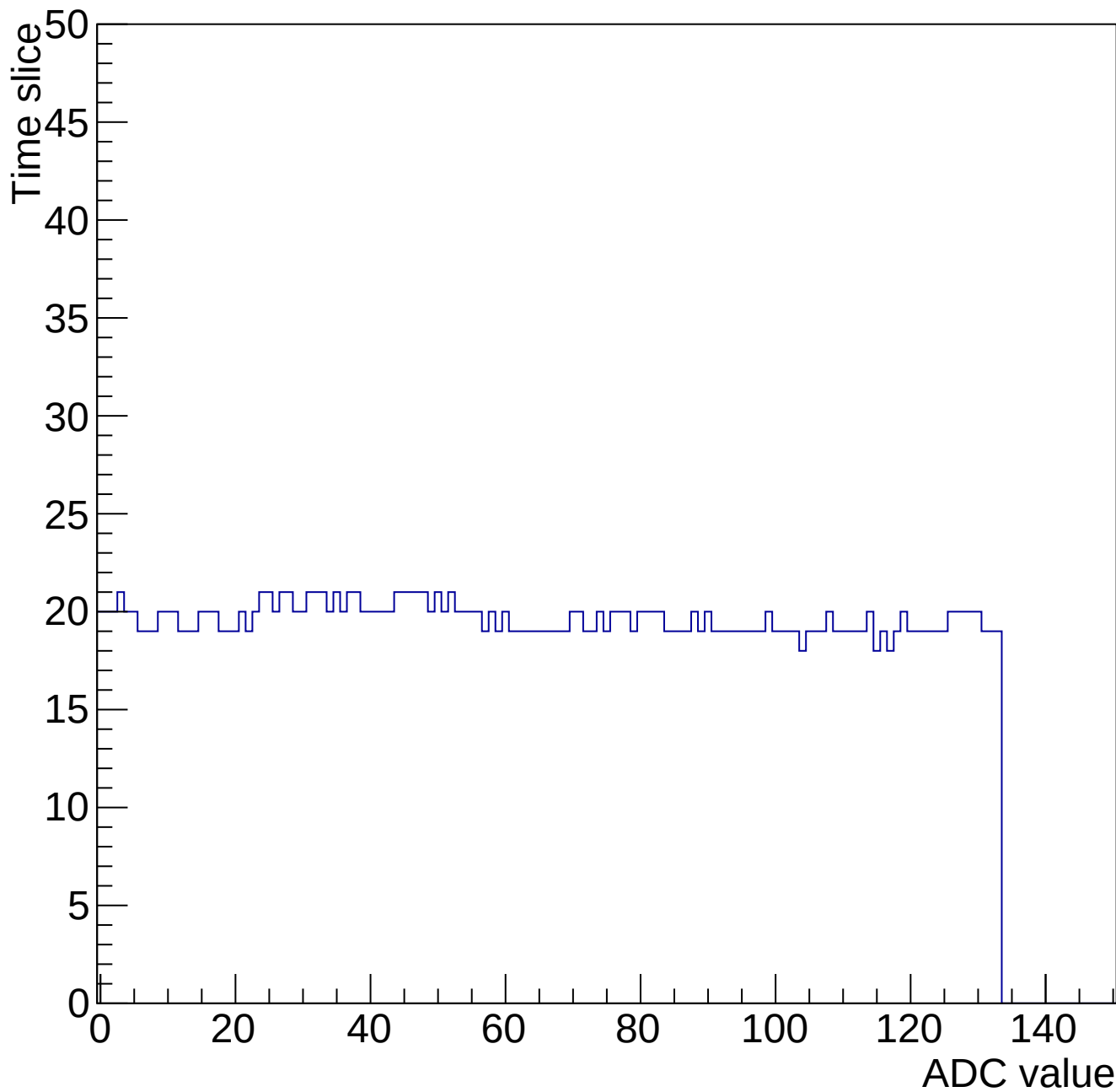
Evt 10 Time mcm 2002 chip 2 chan 11 chip2-nominal-34528
