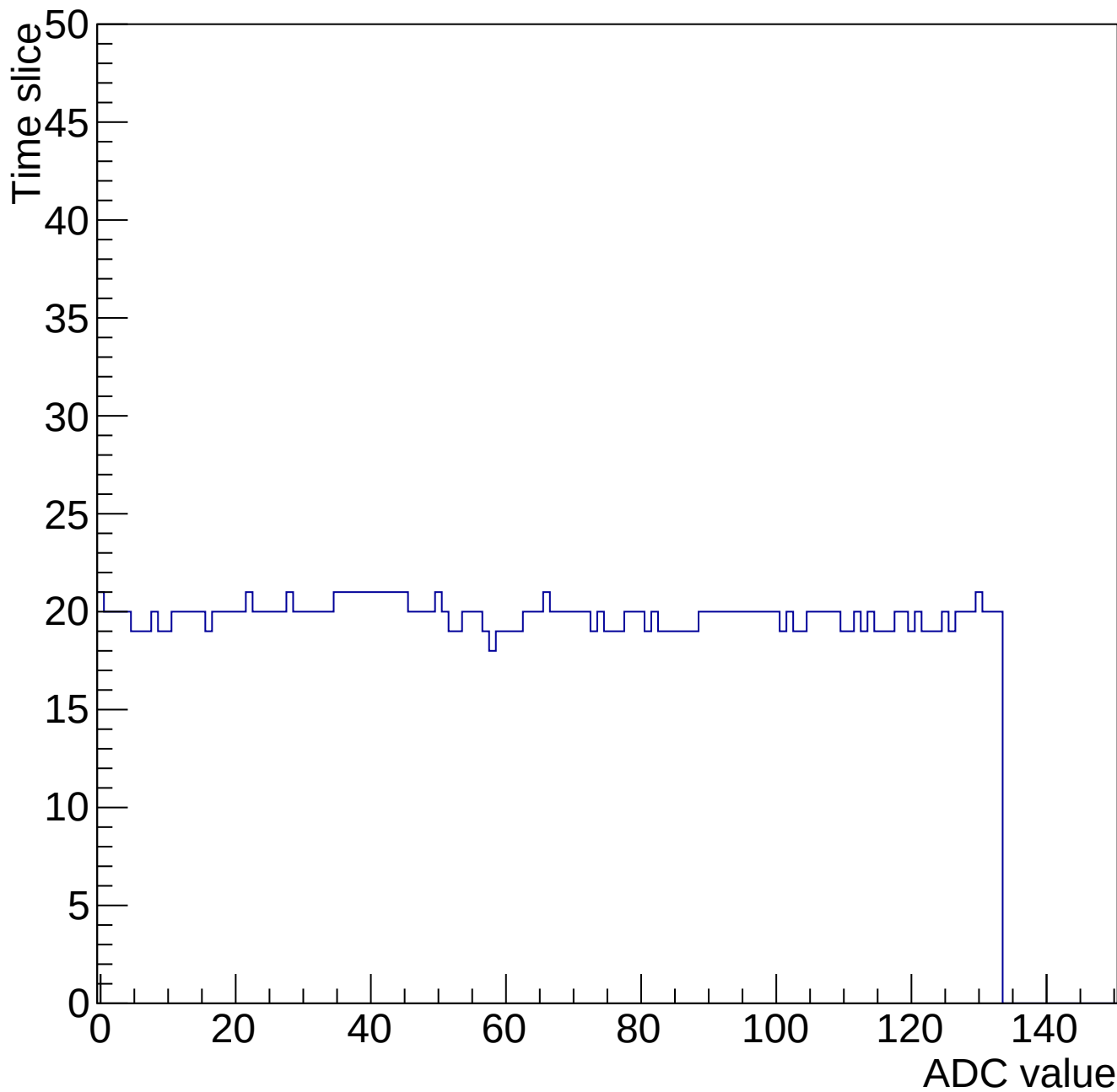
Evt 10 Time mcm 2002 chip 2 chan 13 chip2-nominal-34528
