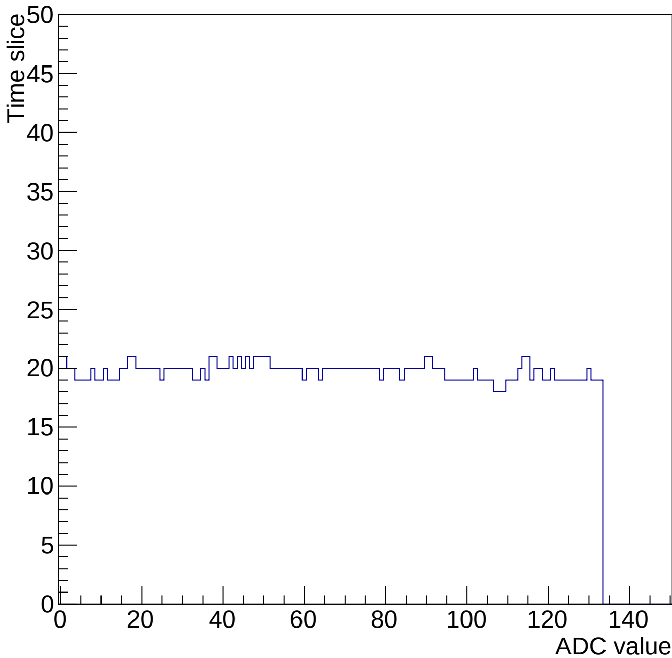
Evt 10 Time mcm 2002 chip 2 chan 9 chip2-nominal-34528
