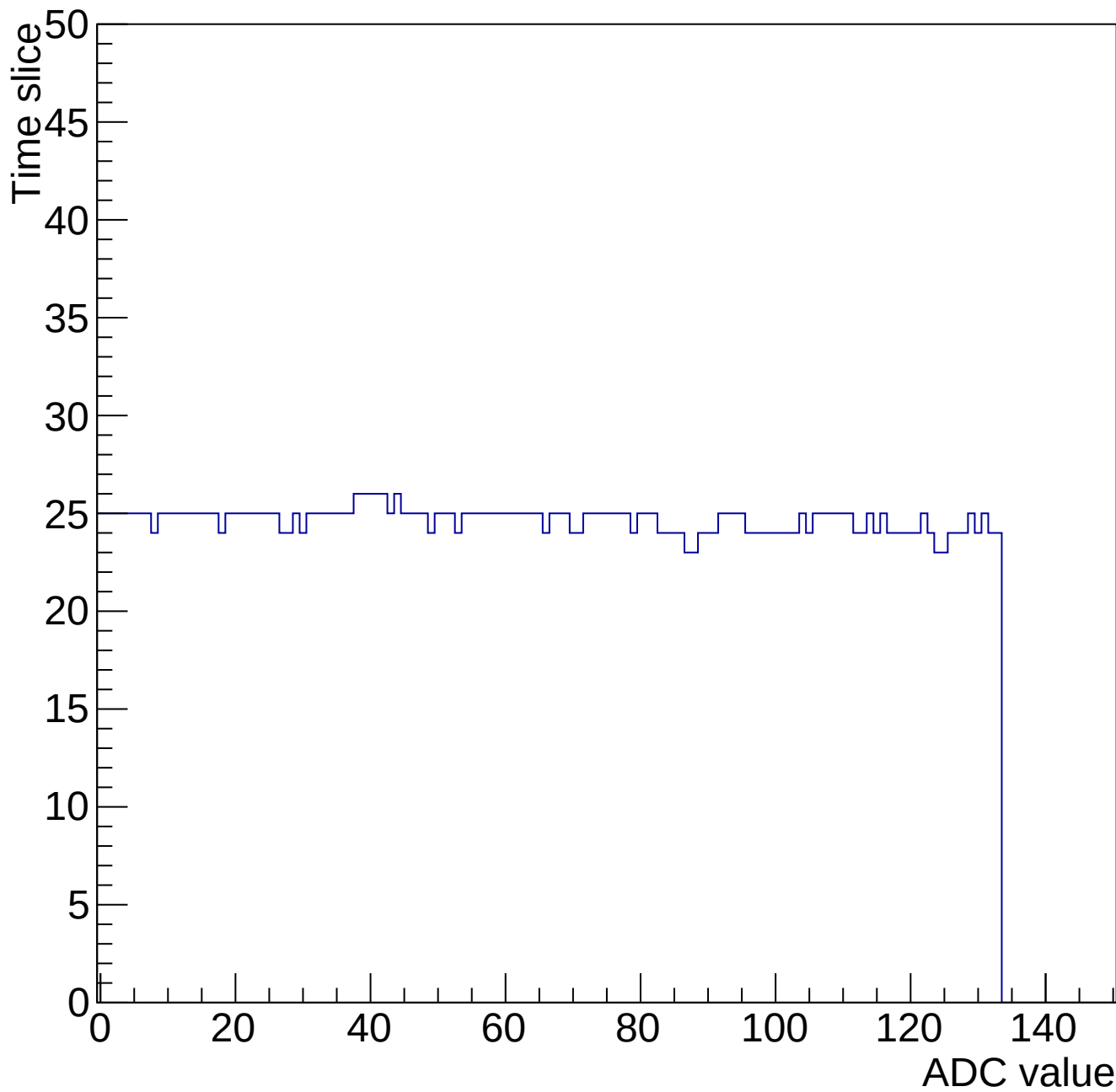
Evt 10 Time mcm 2002 chip 2 chan 5 chip2-nominal-34528
