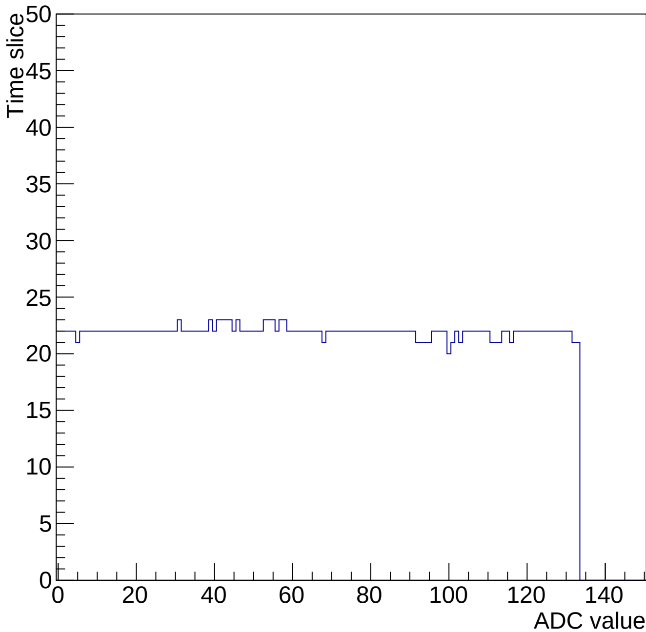
Evt 10 Time mcm 2002 chip 2 chan 7 chip2-nominal-34528
