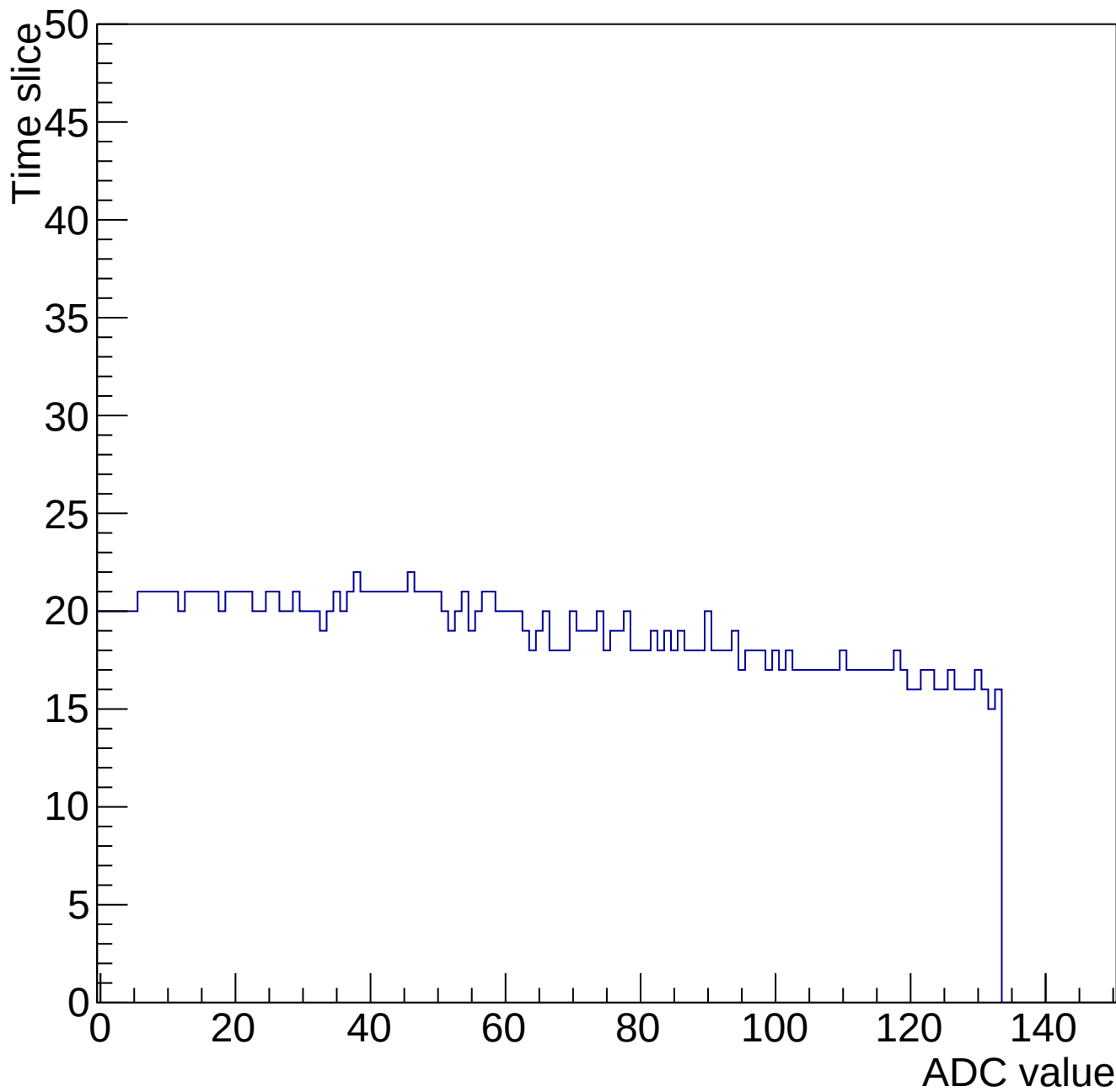
Evt 10 Time mcm 2003 chip 3 chan 8 chip3-nominal-34539
