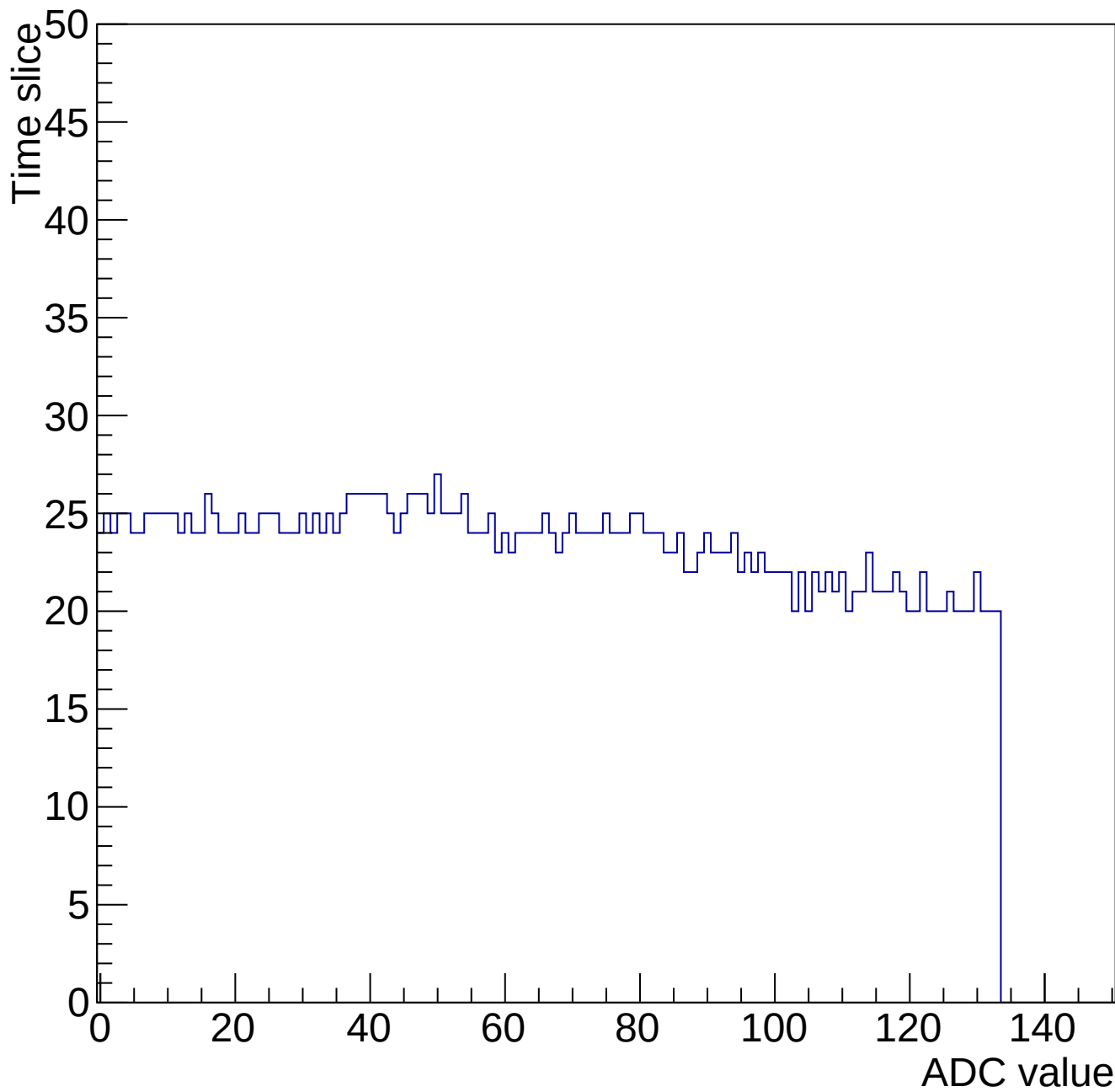
Evt 10 Time mcm 2003 chip 3 chan 9 chip3-nominal-34539
