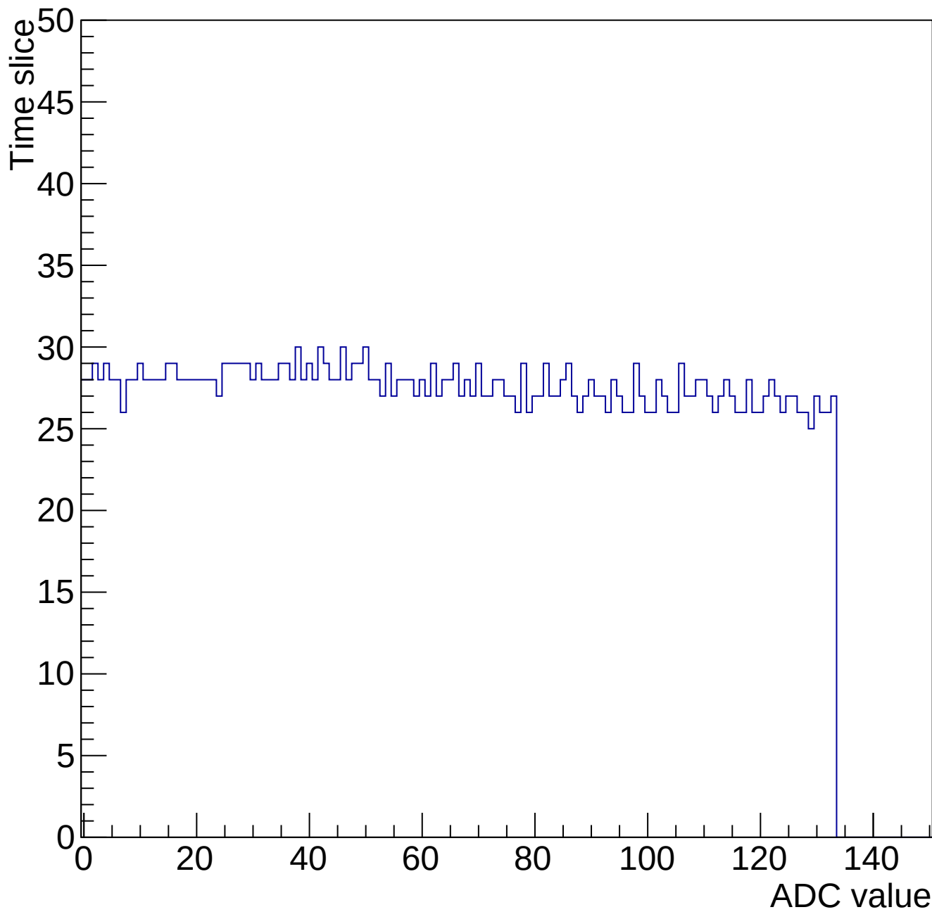
Evt 10 Time mcm 2005 chip 5 chan 0 chip5-nominal-34531
