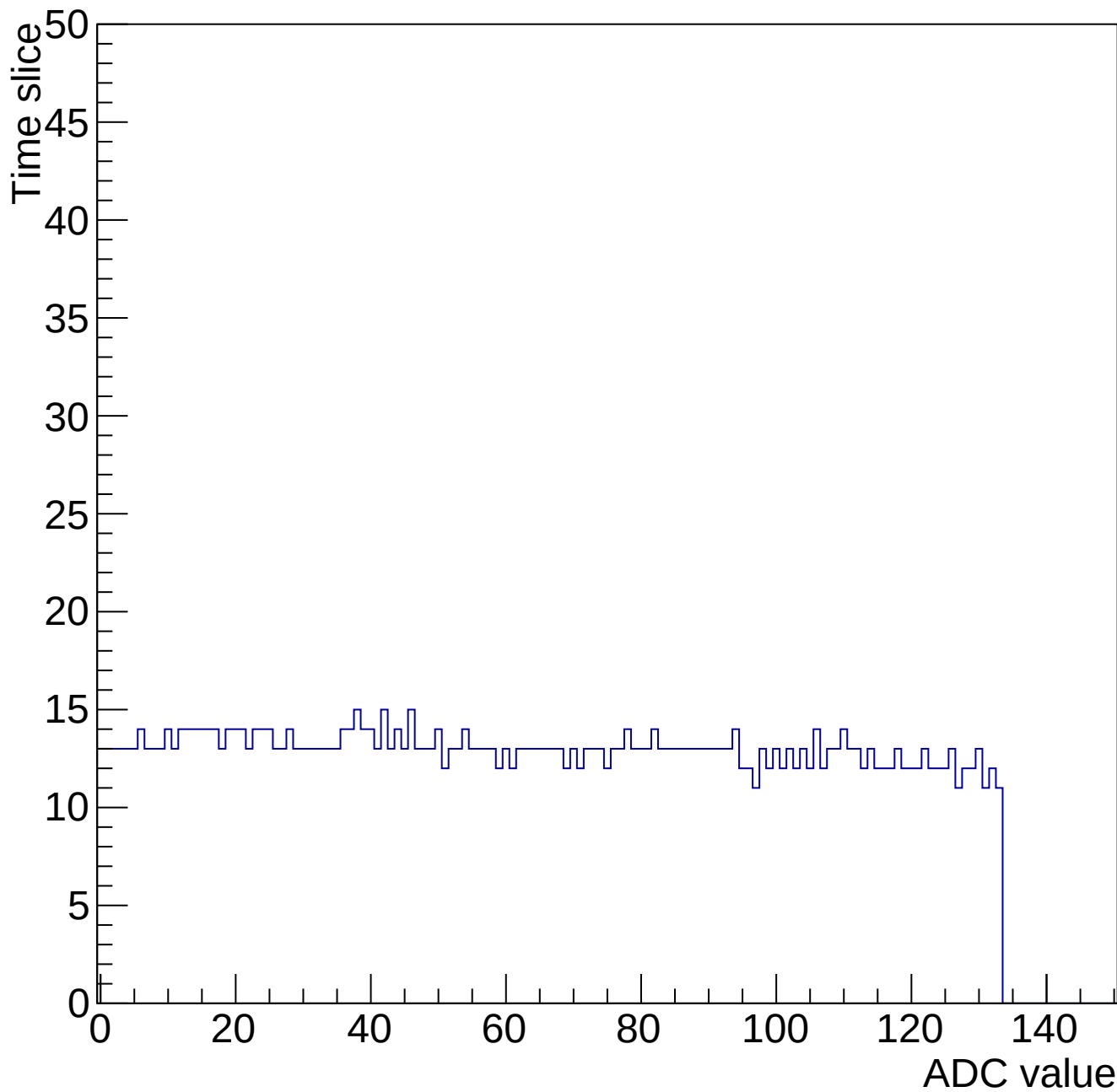
Evt 10 Time mcm 2005 chip 5 chan 4 chip5-nominal-34531
