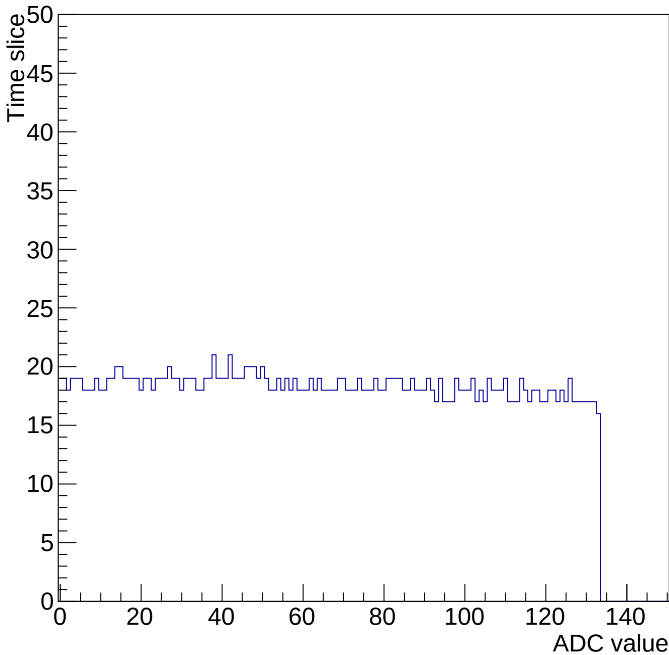
Evt 10 Time mcm 2005 chip 5 chan 14 chip5-nominal-34531
