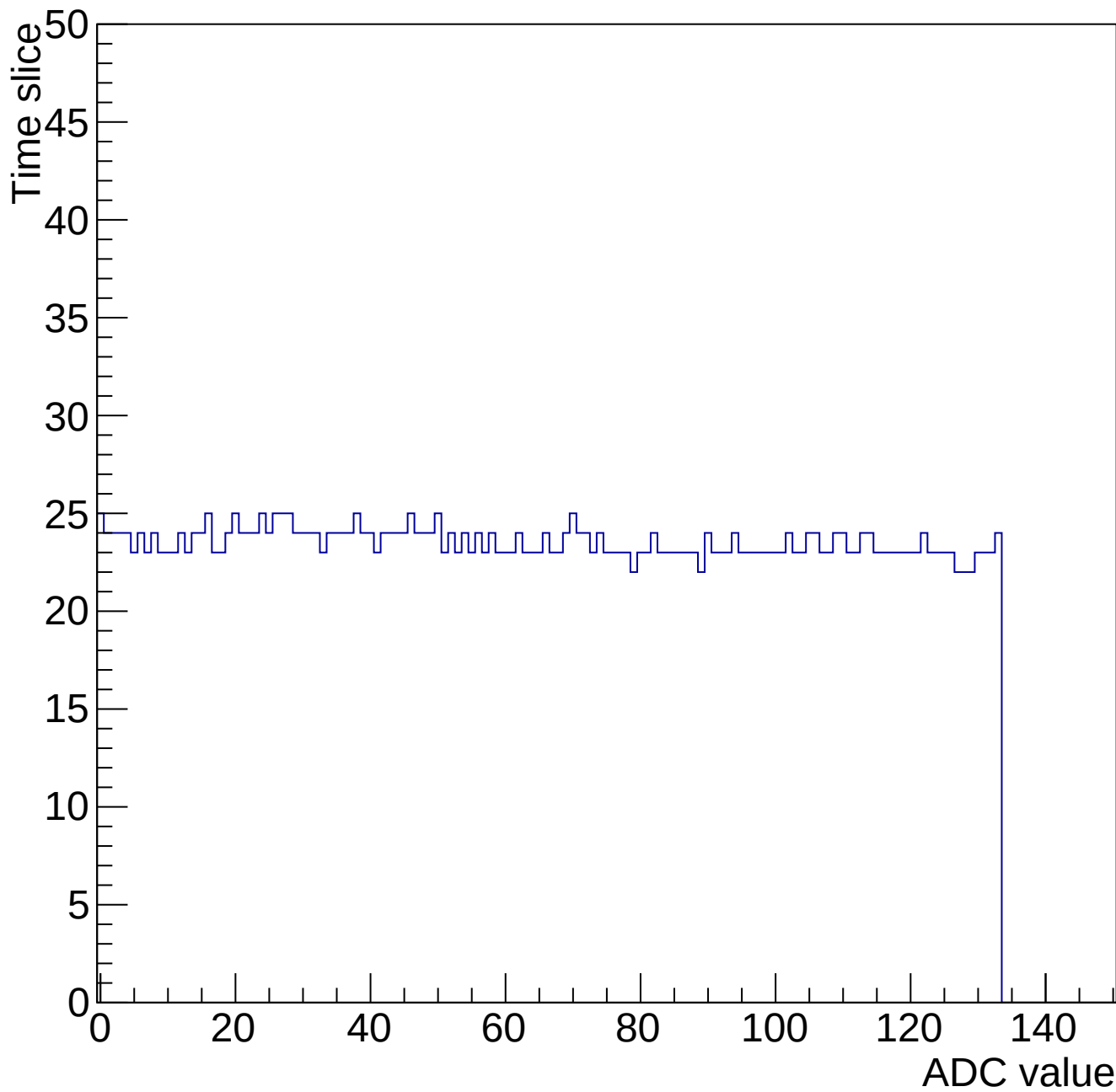
Evt 10 Time mcm 2005 chip 5 chan 8 chip5-nominal-34542
