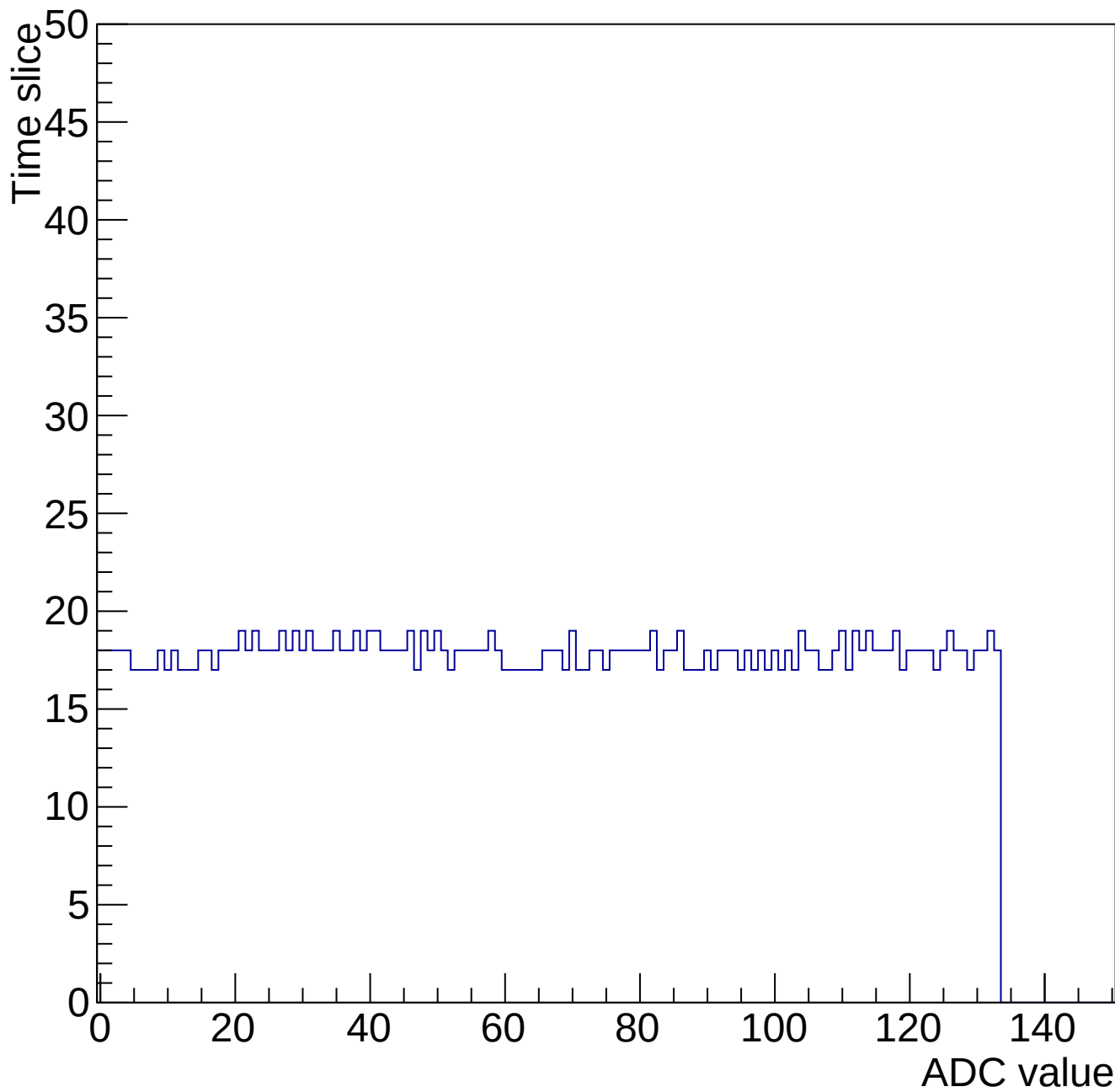
Evt 10 Time mcm 2005 chip 5 chan 11 chip5-nominal-34542
