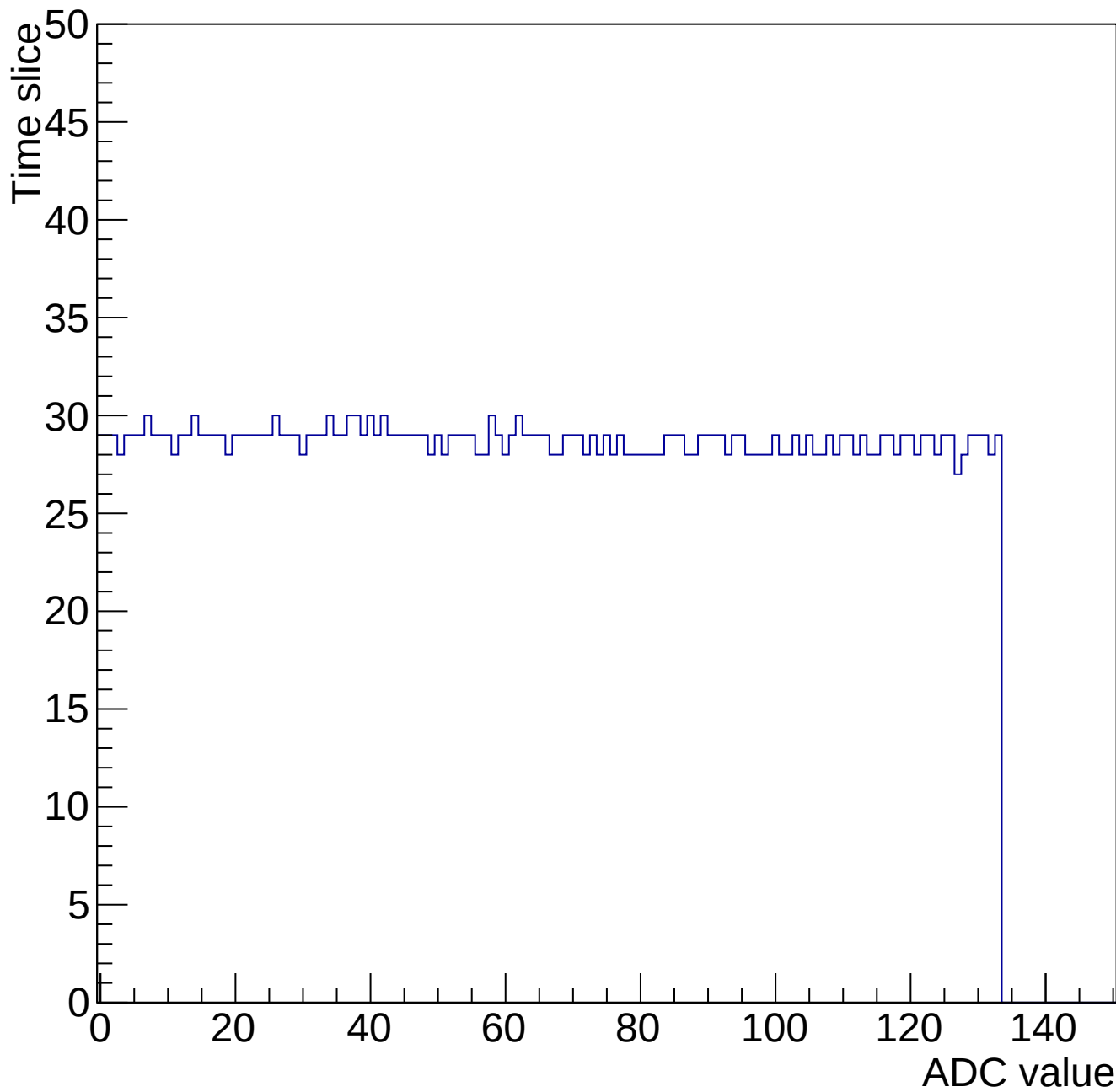
Evt 10 Time mcm 2005 chip 5 chan 3 chip5-nominal-34542
