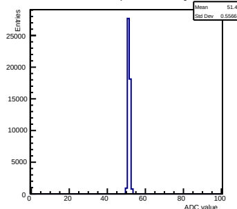
Pedestals ch 14 chip 2000 nominal-gain0
