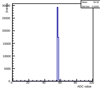
Pedestals ch 1 chip 2000 nominal-gain0
