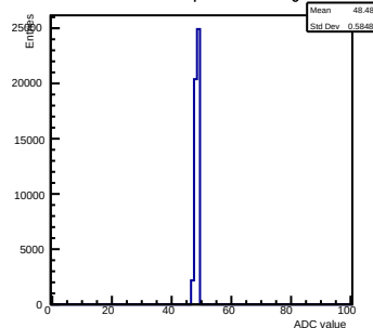
Pedestals ch 11 chip 2000 nominal-gain0
