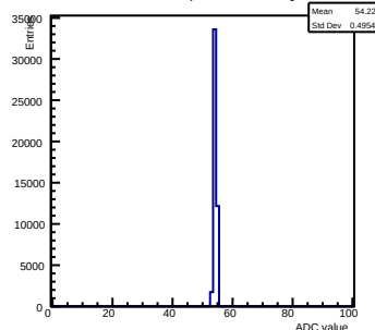
Pedestals ch 7 chip 2000 nominal-gain0
