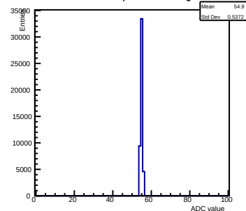
Pedestals ch 8 chip 2000 nominal-gain0
