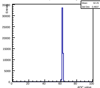
Pedestals ch 5 chip 2000 nominal-gain0
