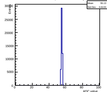
Pedestals ch 12 chip 2000 nominal-gain0
