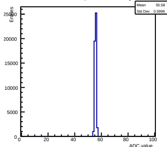
Pedestals ch 13 chip 2000 nominal-gain0
