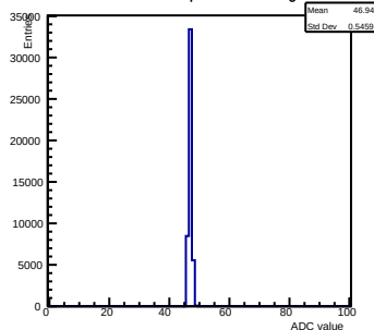
Pedestals ch 10 chip 2000 nominal-gain0
