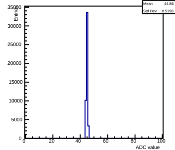
Pedestals ch 0 chip 2000 nominal-gain0
