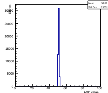
Pedestals ch 4 chip 2000 nominal-gain0
