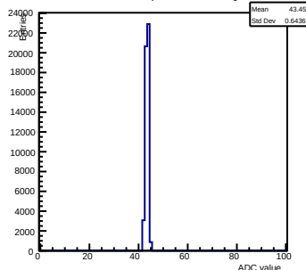
Pedestals ch 6 chip 2000 nominal-gain0
