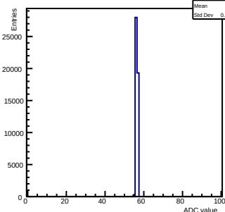
Pedestals ch 12 chip 2000 gain0-shaper6
