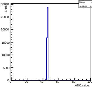
Pedestals ch 0 chip 2000 gain0-shaper6
