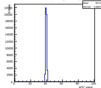
Pedestals ch 4 chip 2000 gain2-shaper0
