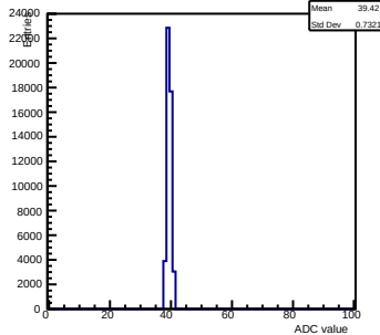
Pedestals ch 2 chip 2000 gain2-shaper0
