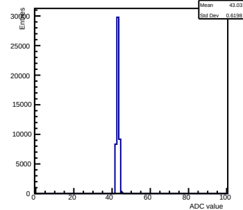
Pedestals ch 8 chip 2000 gain2-shaper0
