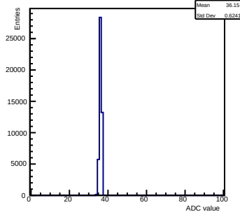
Pedestals ch 10 chip 2000 gain2-shaper0
