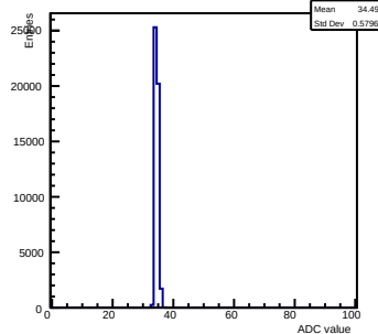
Pedestals ch 15 chip 2000 gain2-shaper0
