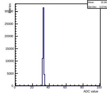
Pedestals ch 0 chip 2000 gain2-shaper0
