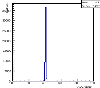
Pedestals ch 14 chip 2000 gain2-shaper0
