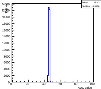
Pedestals ch 13 chip 2000 gain2-shaper0
