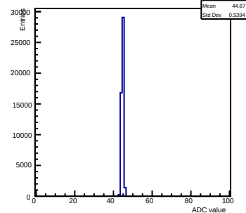
Pedestals ch 12 chip 2000 gain2-shaper0
