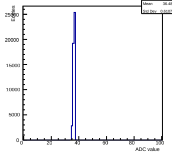
Pedestals ch 11 chip 2000 gain2-shaper0
