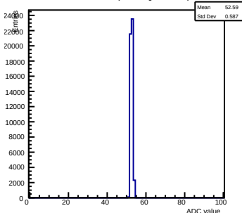
Pedestals ch 5 chip 2000 gain2-shaper0
