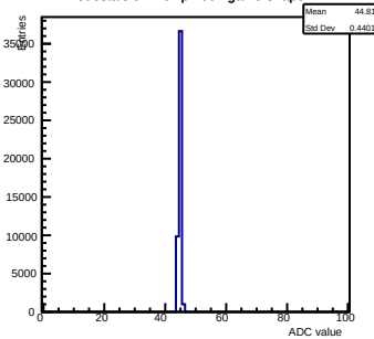
Pedestals ch 2 chip 2001 gain0-shaper4
