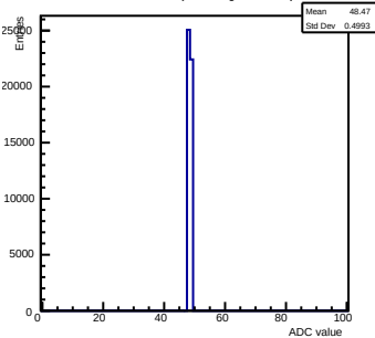
Pedestals ch 5 chip 2001 gain0-shaper4
