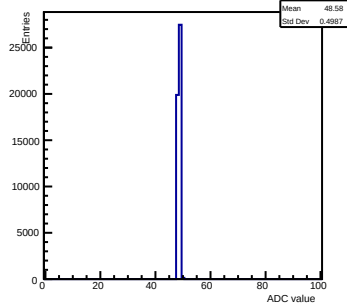
Pedestals ch 12 chip 2001 gain0-shaper4
