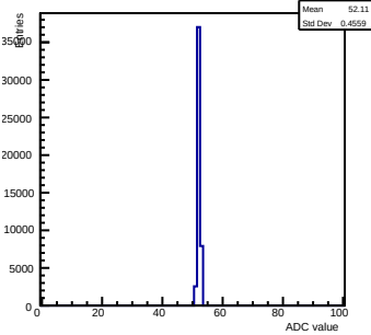
Pedestals ch 13 chip 2001 gain0-shaper4
