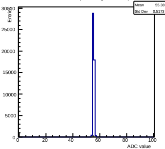
Pedestals ch 6 chip 2001 gain0-shaper4
