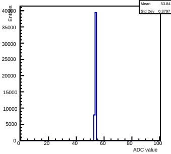
Pedestals ch 11 chip 2001 gain0-shaper4
