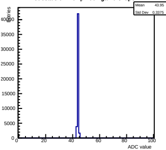
Pedestals ch 1 chip 2001 gain0-shaper4
