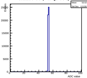
Pedestals ch 3 chip 2001 gain0-shaper4
