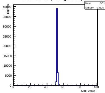
Pedestals ch 0 chip 2001 gain0-shaper4
