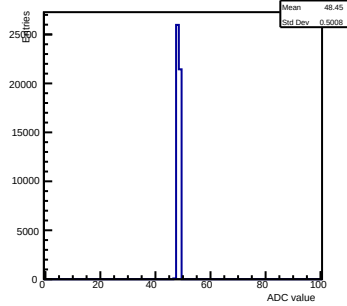
Pedestals ch 8 chip 2001 gain0-shaper4
