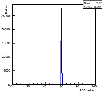
Pedestals ch 15 chip 2001 gain0-shaper7
