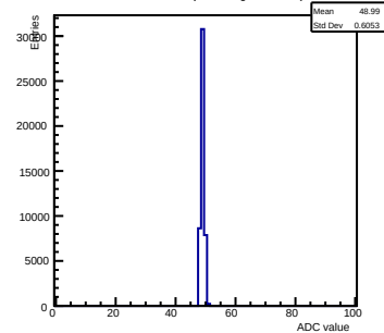
Pedestals ch 12 chip 2001 gain0-shaper7
