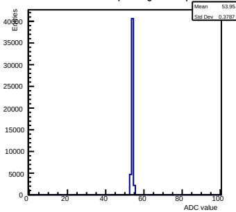
Pedestals ch 11 chip 2001 gain0-shaper7
