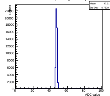
Pedestals ch 4 chip 2001 gain0-shaper7
