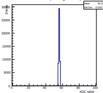
Pedestals ch 6 chip 2001 gain0-shaper7
