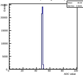
Pedestals ch 5 chip 2001 gain0-shaper7
