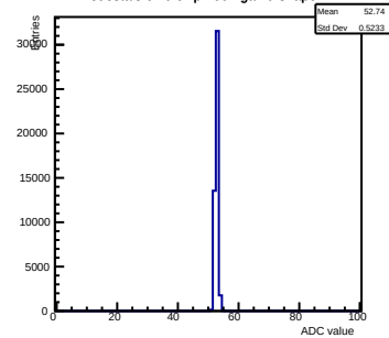
Pedestals ch 0 chip 2001 gain0-shaper7
