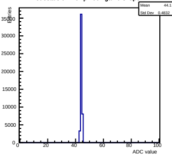
Pedestals ch 1 chip 2001 gain0-shaper7
