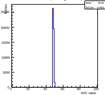
Pedestals ch 9 chip 2001 gain0-shaper7
