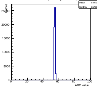
Pedestals ch 10 chip 2001 gain0-shaper7
