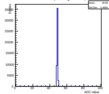
Pedestals ch 8 chip 2001 gain0-shaper7
