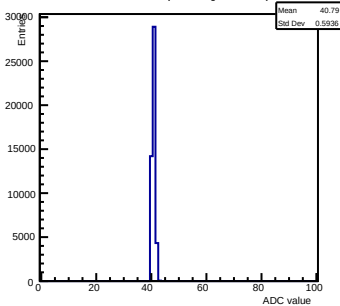
Pedestals ch 14 chip 2001 gain0-shaper7
