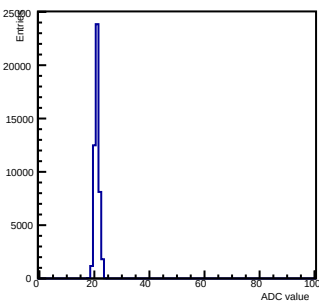
Pedestals ch 0 chip 2001 gain3-shaper7
