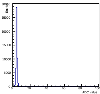
Pedestals ch 1 chip 2001 gain3-shaper7
