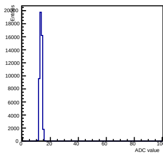
Pedestals ch 2 chip 2001 gain3-shaper7
