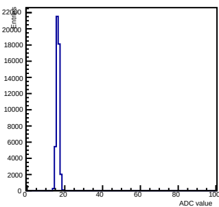
Pedestals ch 8 chip 2001 gain3-shaper7
