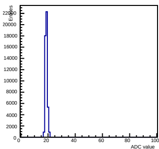
Pedestals ch 13 chip 2001 gain3-shaper7
