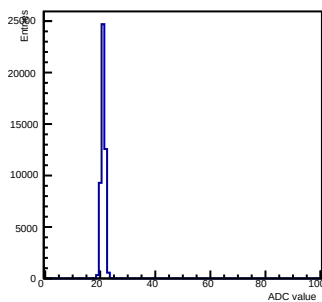
Pedestals ch 3 chip 2001 gain3-shaper7
