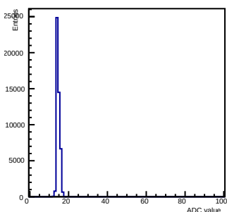
Pedestals ch 5 chip 2001 gain3-shaper7
