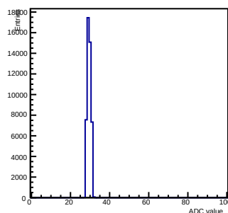
Pedestals ch 6 chip 2001 gain3-shaper7
