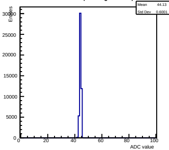
Pedestals ch 11 chip 2001 gain2-shaper7
