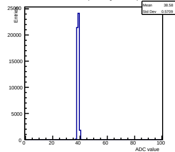
Pedestals ch 12 chip 2001 gain2-shaper7
