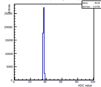
Pedestals ch 4 chip 2001 gain2-shaper7
