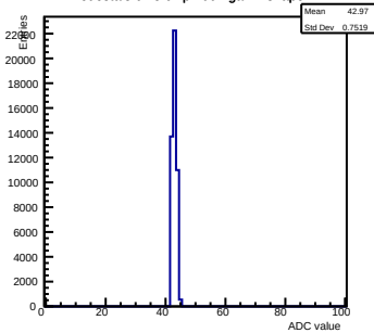
Pedestals ch 3 chip 2001 gain2-shaper7
