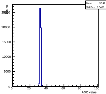
Pedestals ch 7 chip 2001 gain2-shaper7
