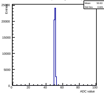
Pedestals ch 15 chip 2001 gain2-shaper7
