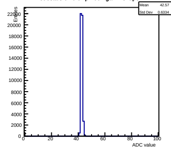
Pedestals ch 0 chip 2001 gain2-shaper7
