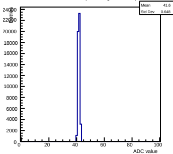
Pedestals ch 13 chip 2001 gain2-shaper7
