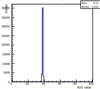
Pedestals ch 5 chip 2001 gain2-shaper7
