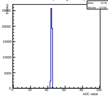
Pedestals ch 10 chip 2001 gain2-shaper7
