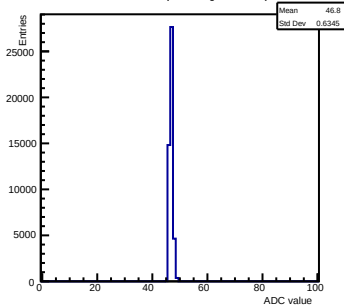
Pedestals ch 6 chip 2001 gain2-shaper7
