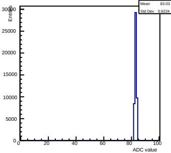
Pedestals ch 11 chip 2001 gain0-shaper0
