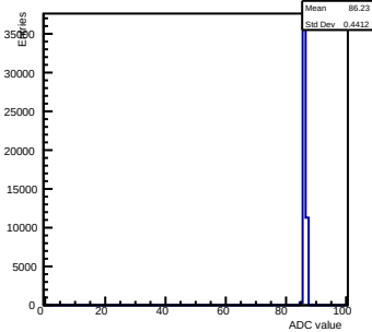
Pedestals ch 3 chip 2001 gain0-shaper0
