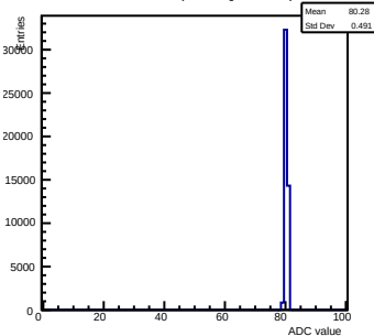
Pedestals ch 5 chip 2001 gain0-shaper0
