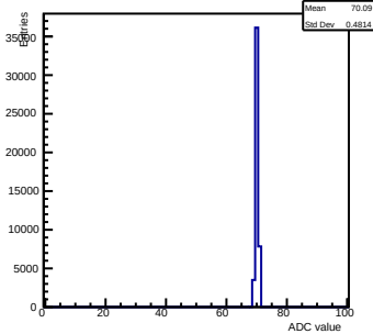
Pedestals ch 2 chip 2001 gain0-shaper0
