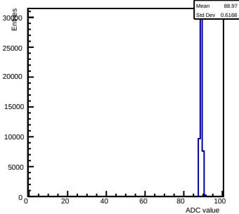
Pedestals ch 15 chip 2001 gain0-shaper0
