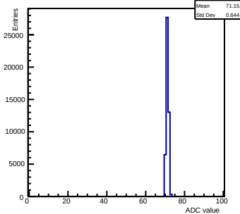
Pedestals ch 14 chip 2001 gain0-shaper0
