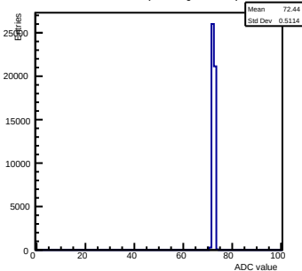
Pedestals ch 7 chip 2001 gain0-shaper0
