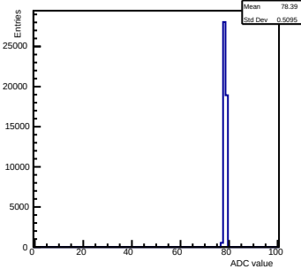
Pedestals ch 8 chip 2001 gain0-shaper0
