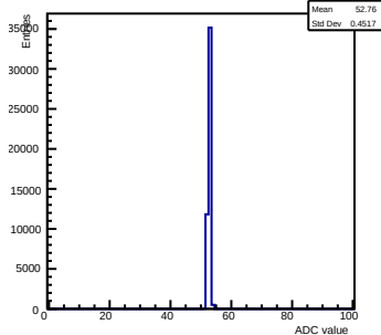
Pedestals ch 5 chip 2002 gain0-shaper7
