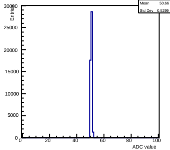
Pedestals ch 11 chip 2002 gain0-shaper7
