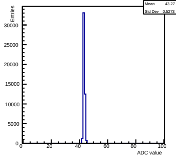
Pedestals ch 3 chip 2002 gain0-shaper7
