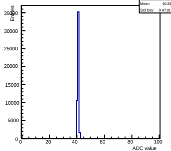
Pedestals ch 14 chip 2002 gain0-shaper7
