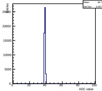
Pedestals ch 2 chip 2002 gain0-shaper7
