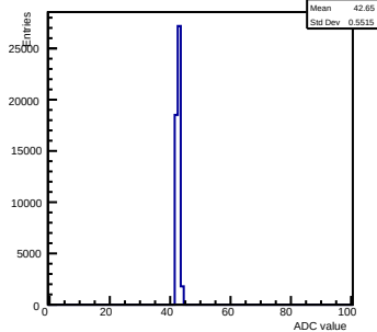
Pedestals ch 15 chip 2002 gain0-shaper7
