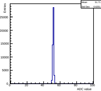
Pedestals ch 0 chip 2002 gain0-shaper7
