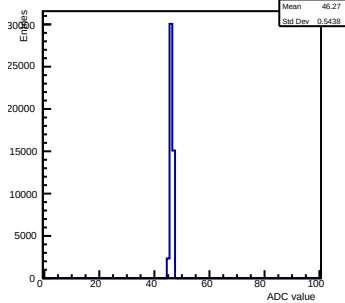
Pedestals ch 9 chip 2002 gain0-shaper7
