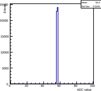
Pedestals ch 4 chip 2002 gain0-shaper7
