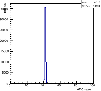
Pedestals ch 12 chip 2002 gain0-shaper7
