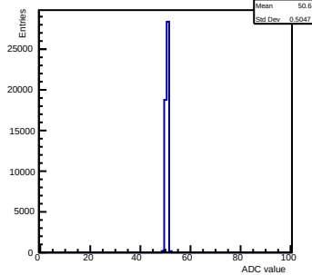
Pedestals ch 10 chip 2002 gain0-shaper7
