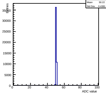
Pedestals ch 13 chip 2002 gain0-shaper7
