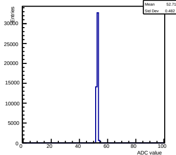
Pedestals ch 7 chip 2002 gain0-shaper7
