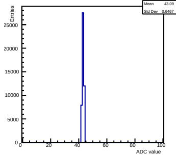
Pedestals ch 1 chip 2002 gain0-shaper7
