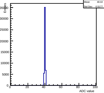
Pedestals ch 8 chip 2002 gain0-shaper7
