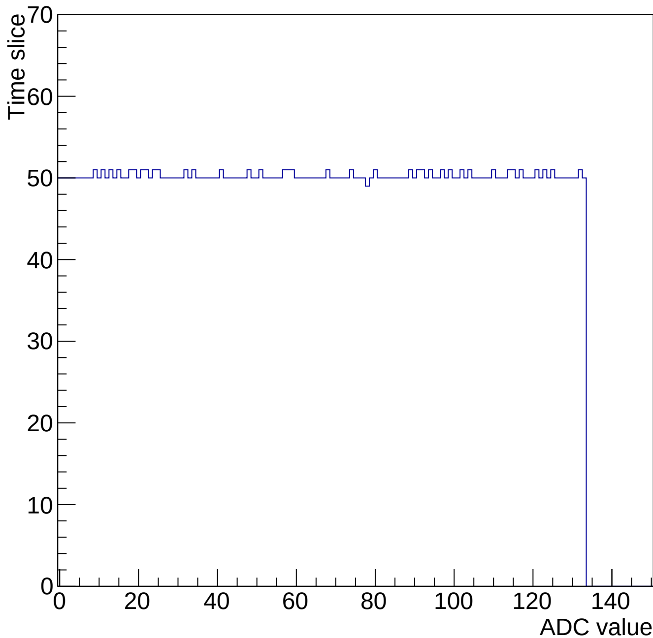
Evt 10 Time mcm 2000 chip 0 chan 3 gain0-shaper0
