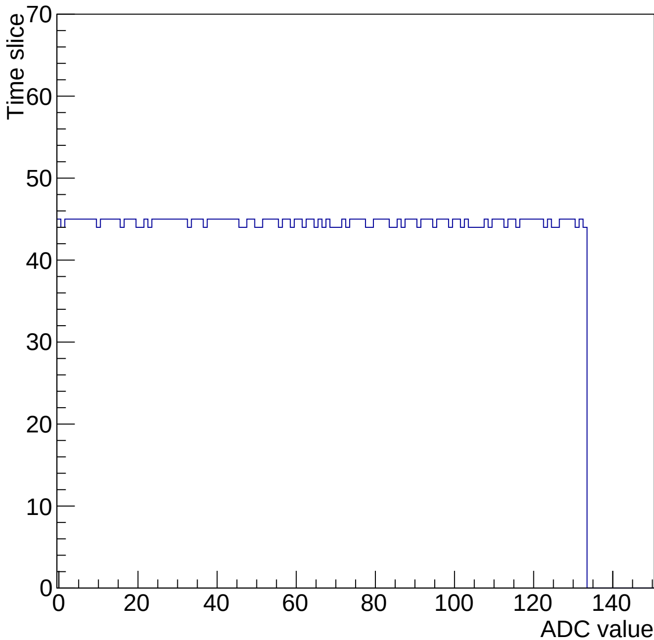
Evt 10 Time mcm 2000 chip 0 chan 9 gain0-shaper0
