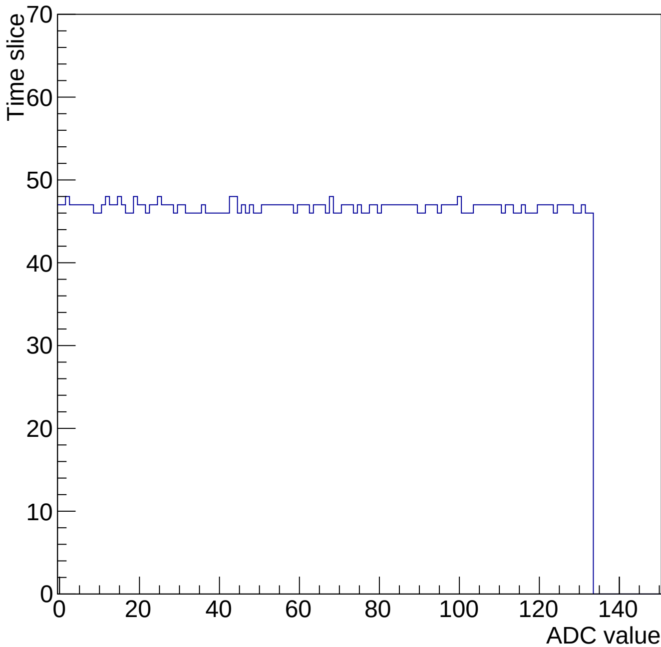
Evt 10 Time mcm 2000 chip 0 chan 15 gain0-shaper0
