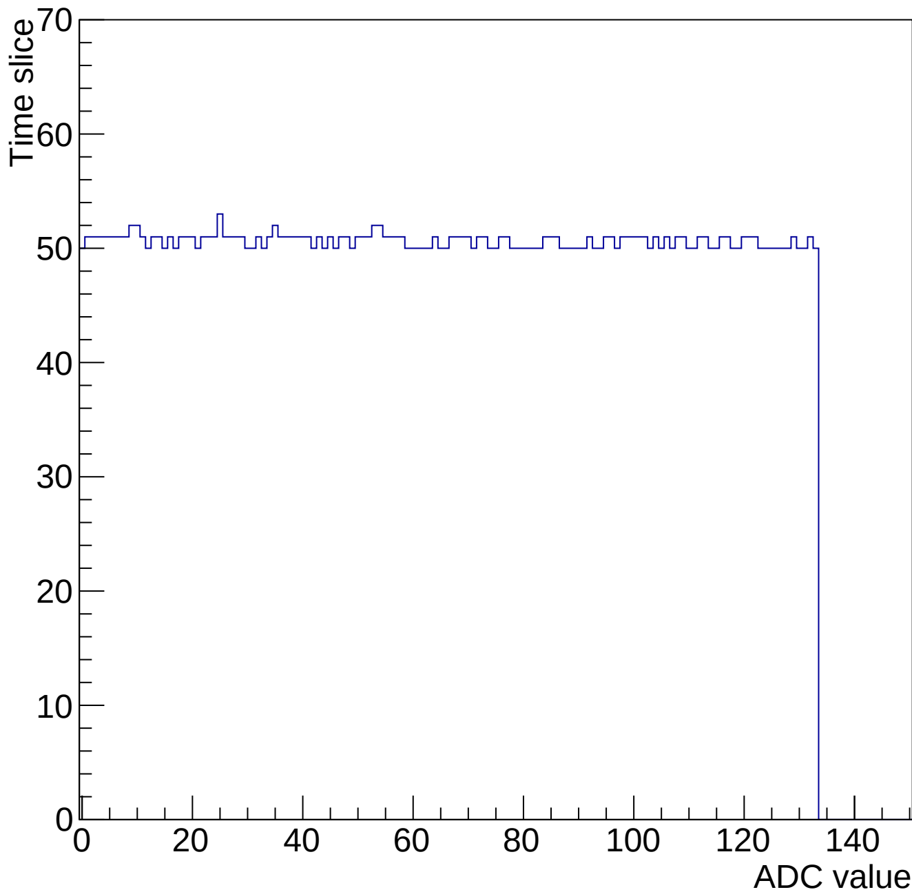
Evt 10 Time mcm 2000 chip 0 chan 4 gain0-shaper0
