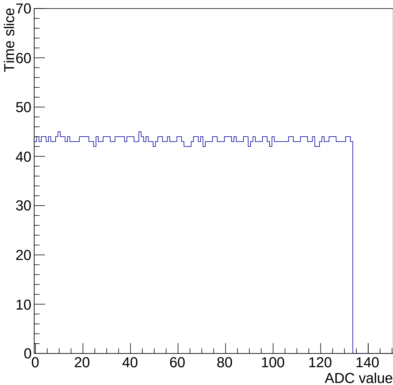
Evt 10 Time mcm 2000 chip 0 chan 6 gain0-shaper0
