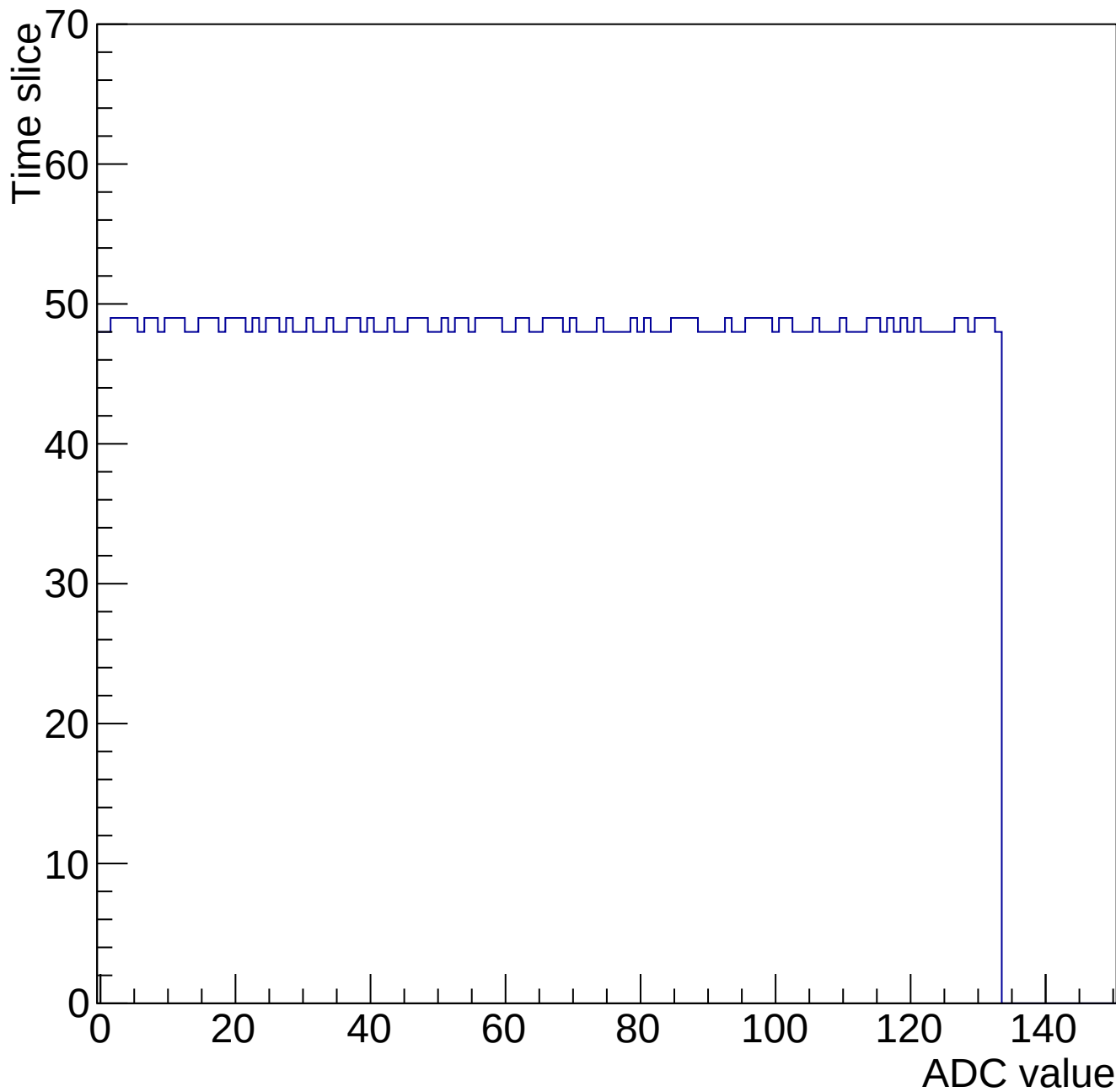
Evt 10 Time mcm 2001 chip 1 chan 5 gain0-shaper7
