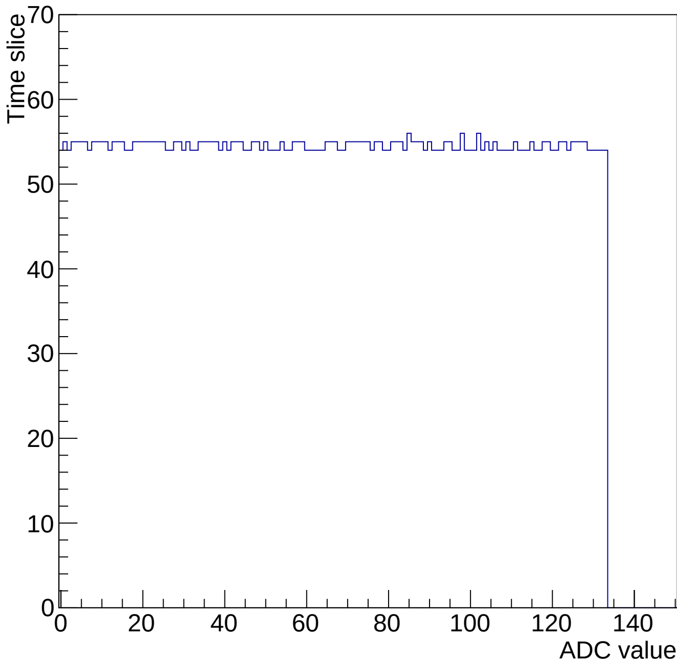
Evt 10 Time mcm 2001 chip 1 chan 10 gain0-shaper7
