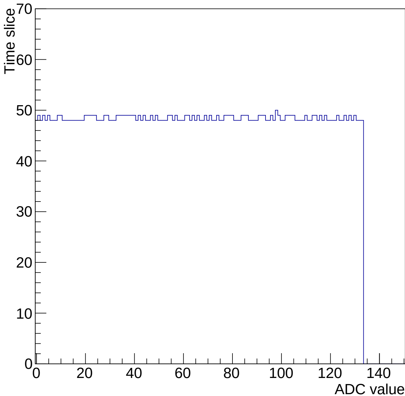
Evt 10 Time mcm 2001 chip 1 chan 9 gain0-shaper7
