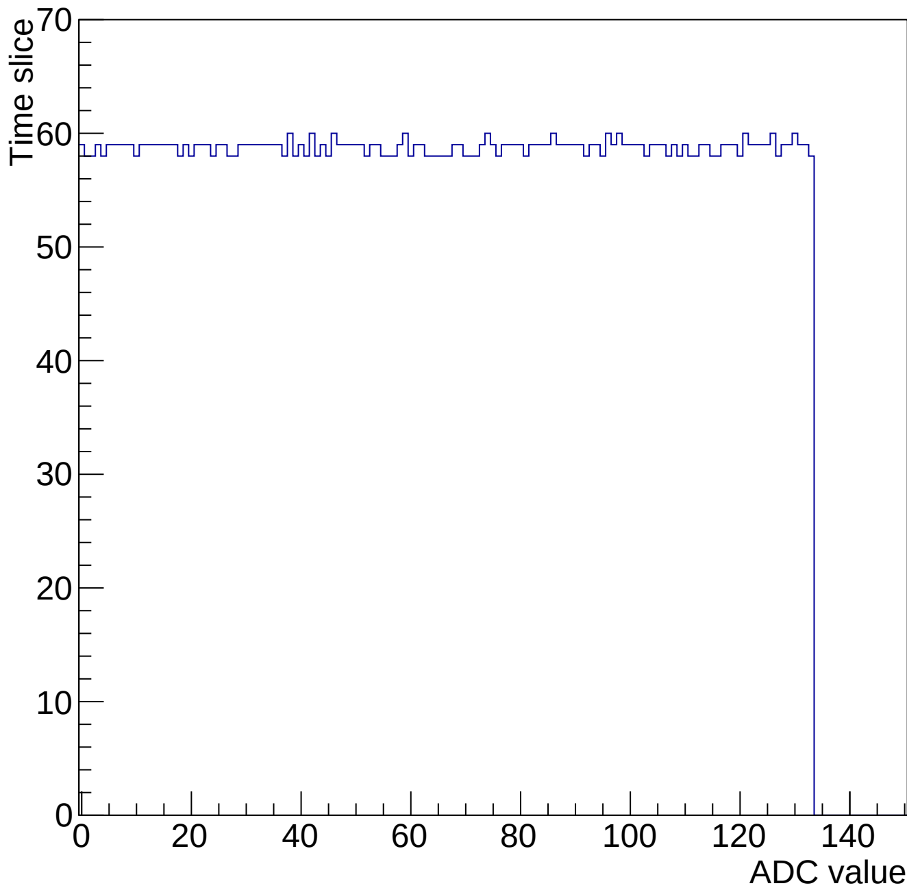
Evt 10 Time mcm 2001 chip 1 chan 15 gain0-shaper7
