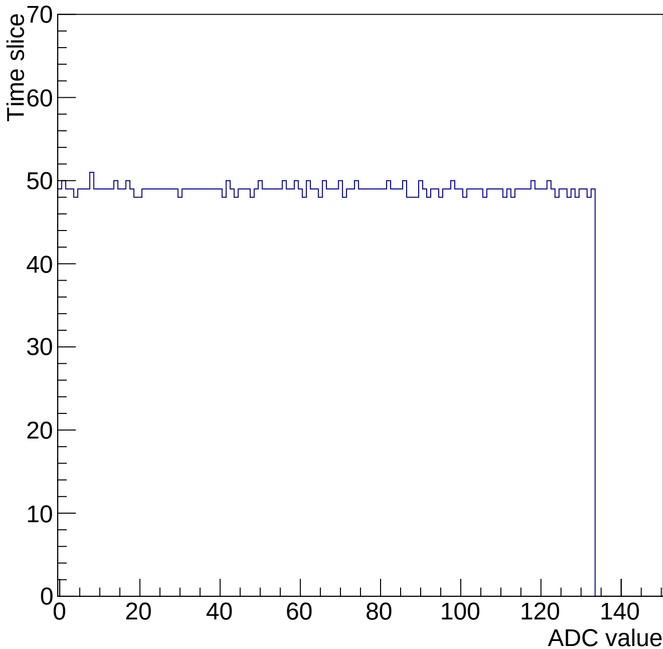
Evt 10 Time mcm 2001 chip 1 chan 12 gain0-shaper7
