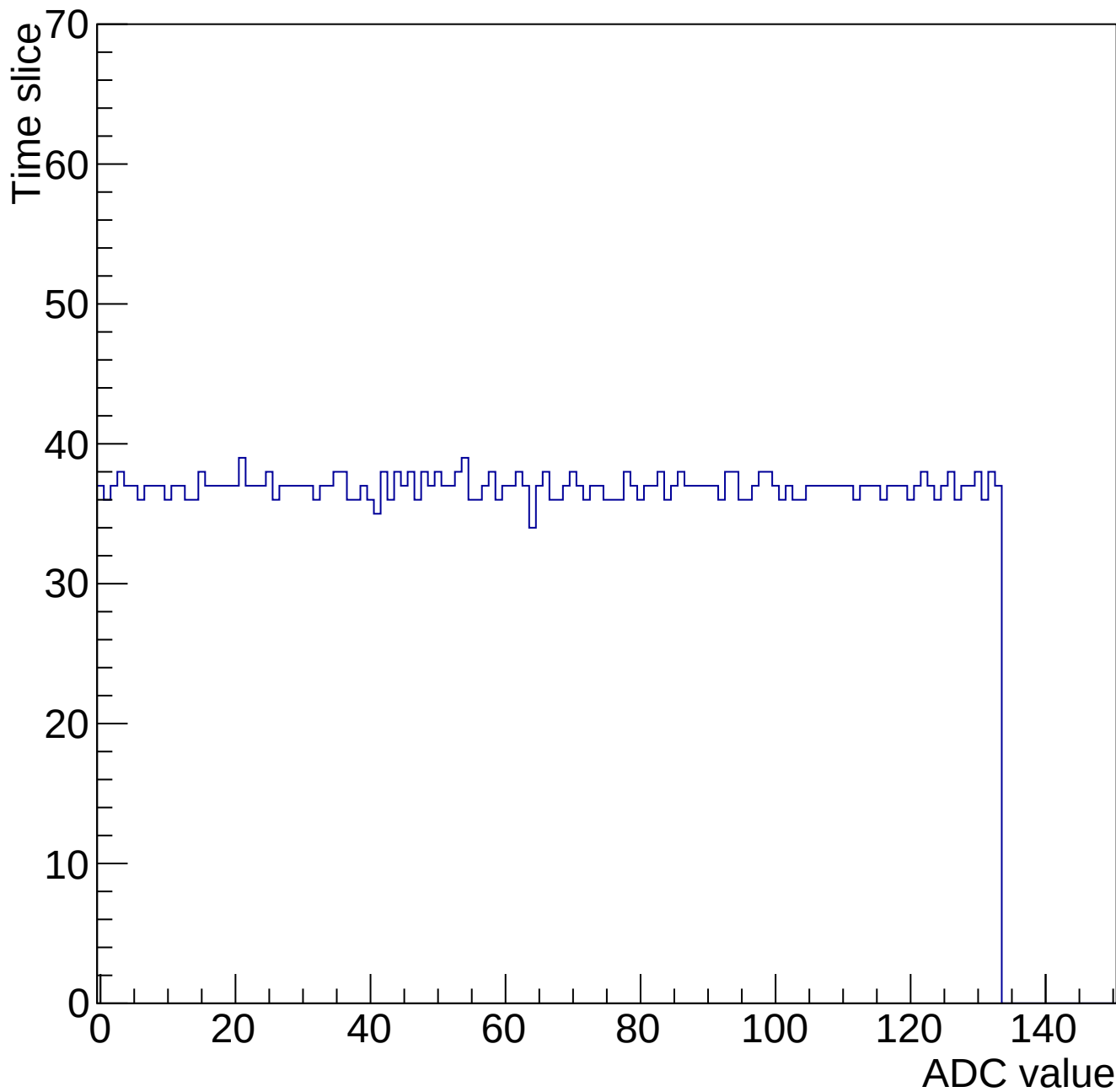
Evt 10 Time mcm 2001 chip 1 chan 15 gain3-shaper7
