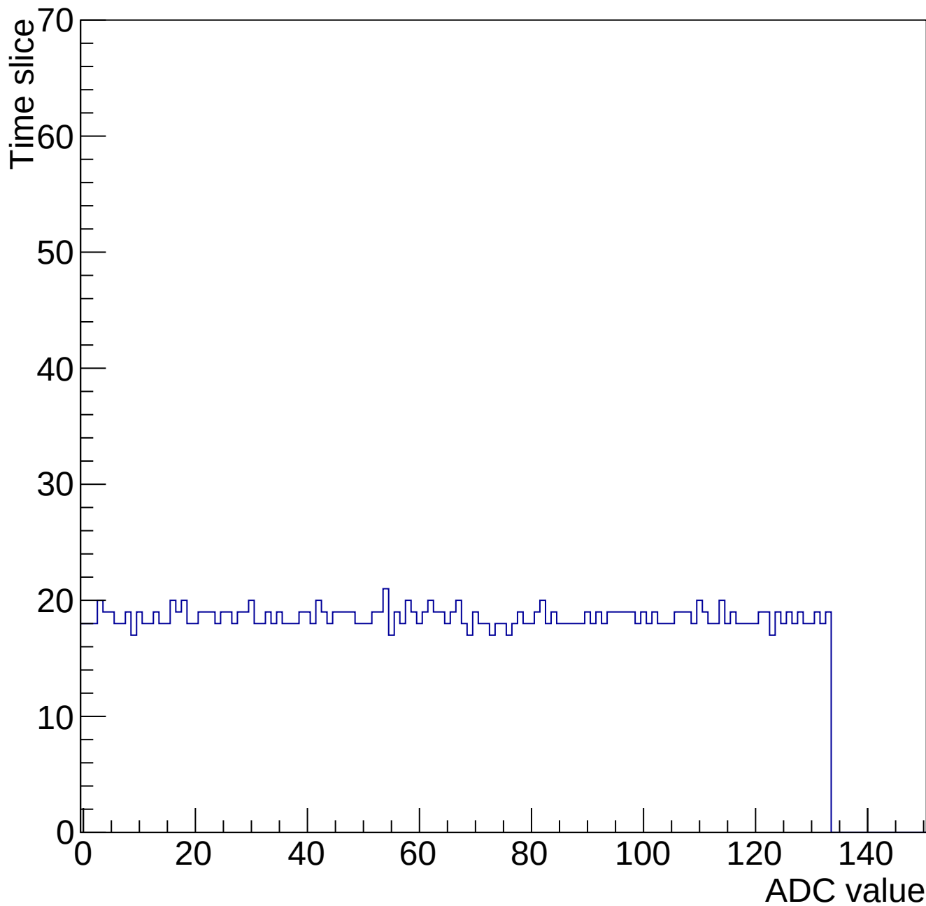
Evt 10 Time mcm 2001 chip 1 chan 13 gain3-shaper7
