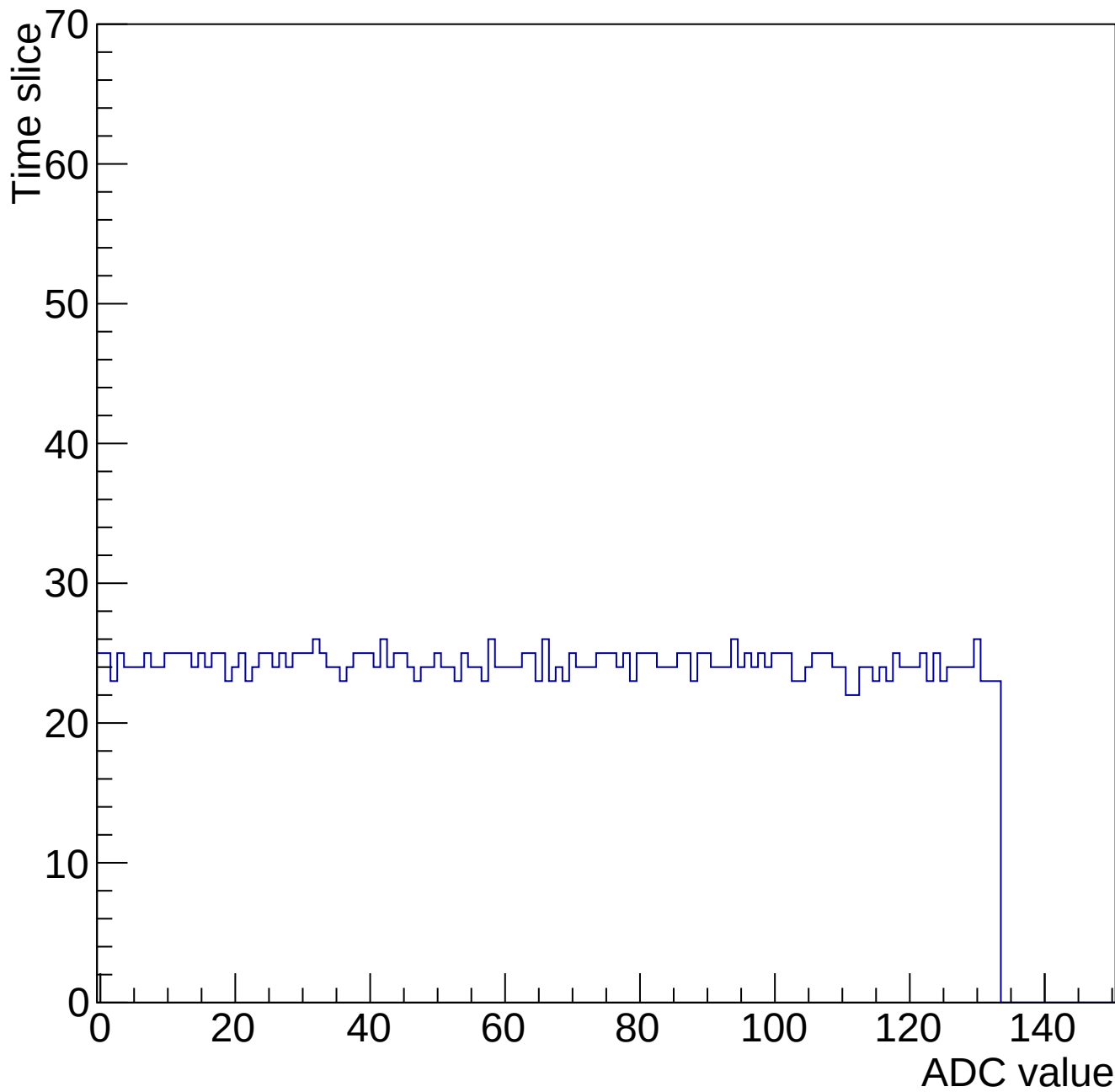
Evt 10 Time mcm 2001 chip 1 chan 10 gain3-shaper7
