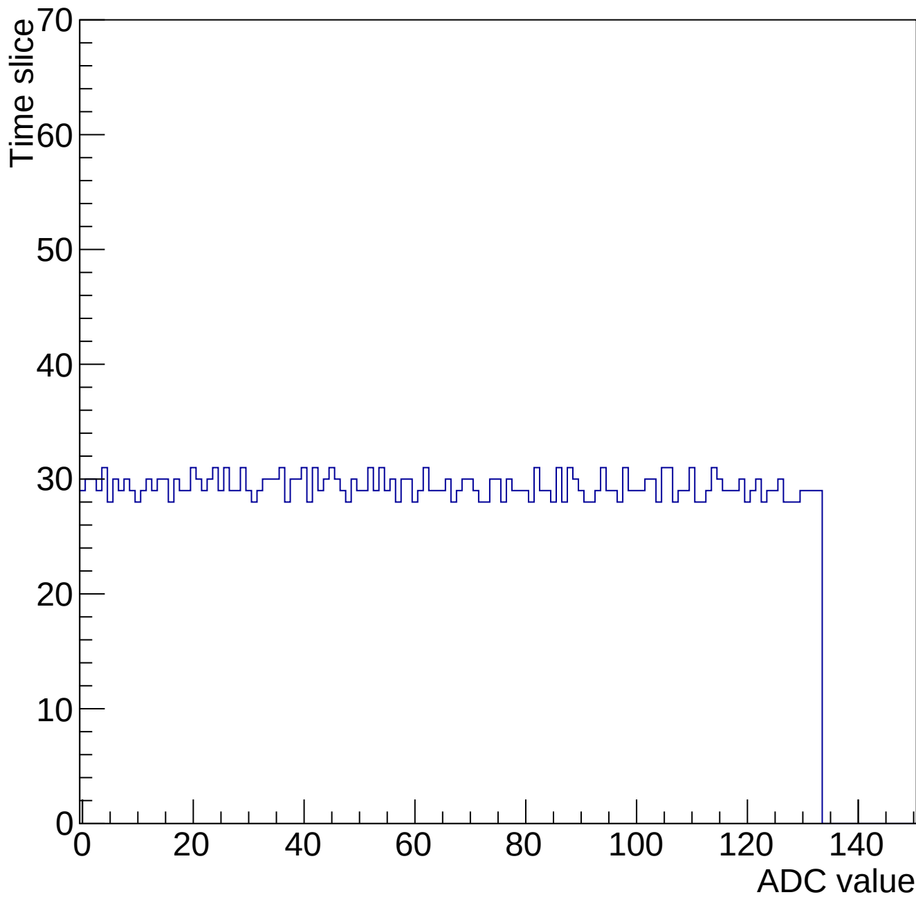
Evt 10 Time mcm 2001 chip 1 chan 6 gain3-shaper7
