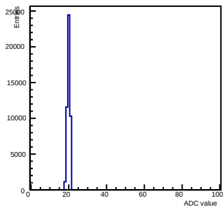
Pedestals ch 15 chip 2000 gain0-shaper0
