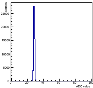
Pedestals ch 8 chip 2000 gain0-shaper0
