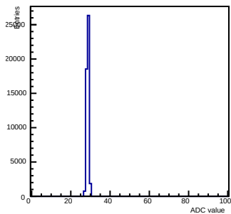
Pedestals ch 13 chip 2000 gain0-shaper0
