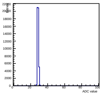
Pedestals ch 1 chip 2000 gain0-shaper0
