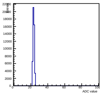
Pedestals ch 3 chip 2000 gain0-shaper0
