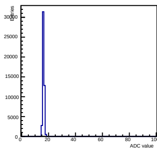
Pedestals ch 6 chip 2000 gain0-shaper0
