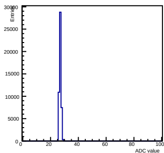
Pedestals ch 7 chip 2000 gain0-shaper0
