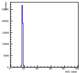
Pedestals ch 9 chip 2000 gain0-shaper0
