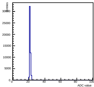
Pedestals ch 11 chip 2000 gain0-shaper0
