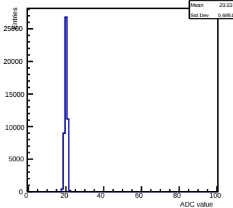
Pedestals ch 10 chip 2000 gain0-shaper0
