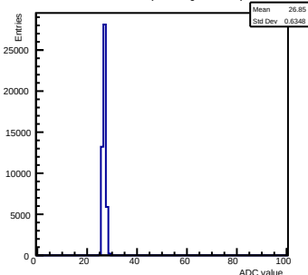
Pedestals ch 7 chip 2000 gain0-shaper0
