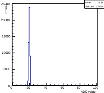
Pedestals ch 15 chip 2000 gain0-shaper0
