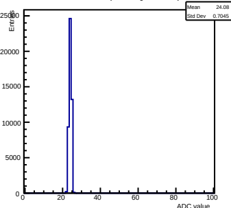
Pedestals ch 4 chip 2000 gain0-shaper0
