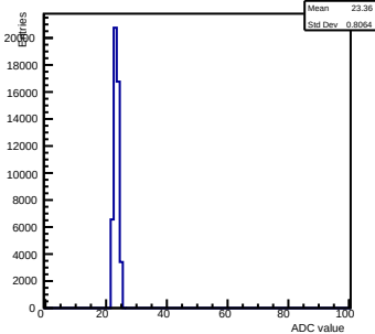
Pedestals ch 3 chip 2000 gain0-shaper0
