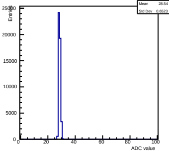
Pedestals ch 1 chip 2000 gain0-shaper0
