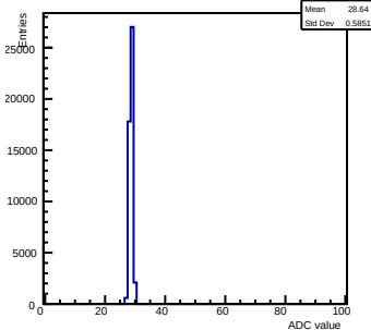
Pedestals ch 13 chip 2000 gain0-shaper0
