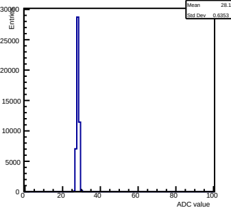
Pedestals ch 8 chip 2000 gain0-shaper0
