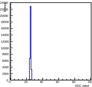
Pedestals ch 12 chip 2000 gain0-shaper7
