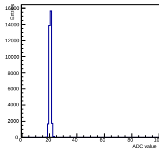
Pedestals ch 2 chip 2000 gain0-shaper7
