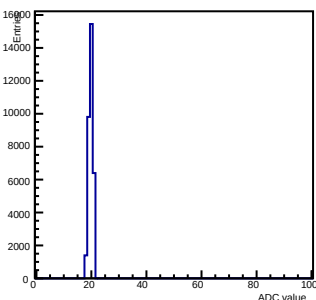
Pedestals ch 4 chip 2000 gain0-shaper7
