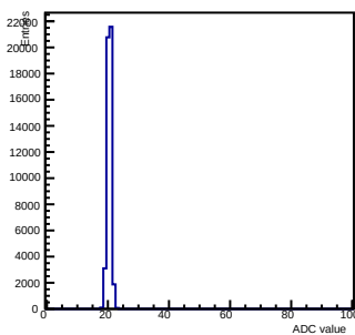
Pedestals ch 2 chip 2000 gain0-shaper7
