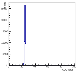
Pedestals ch 8 chip 2000 gain0-shaper7
