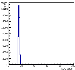
Pedestals ch 0 chip 2000 gain0-shaper7
