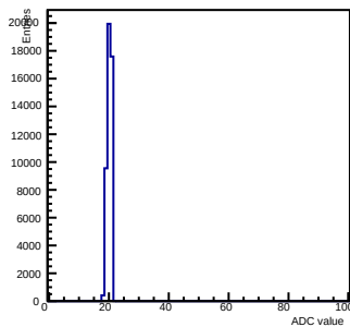
Pedestals ch 11 chip 2000 gain0-shaper7
