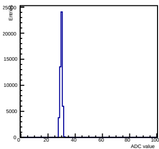
Pedestals ch 1 chip 2000 gain0-shaper7
