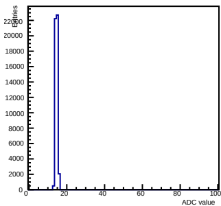
Pedestals ch 9 chip 2000 gain0-shaper7
