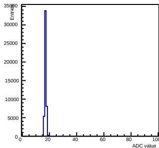
Pedestals ch 15 chip 2000 gain0-shaper7
