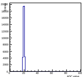
Pedestals ch 4 chip 2000 gain0-shaper7
