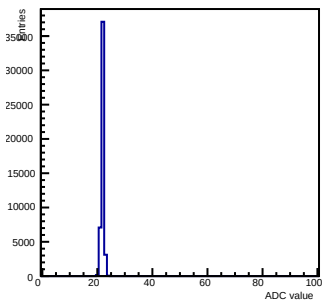
Pedestals ch 13 chip 2000 gain0-shaper7
