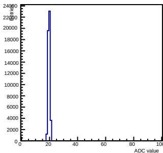
Pedestals ch 14 chip 2000 gain0-shaper7
