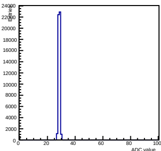
Pedestals ch 12 chip 2000 gain0-shaper0
