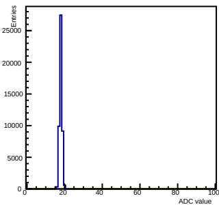
Pedestals ch 0 chip 2000 gain0-shaper0
