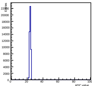
Pedestals ch 4 chip 2000 gain0-shaper0
