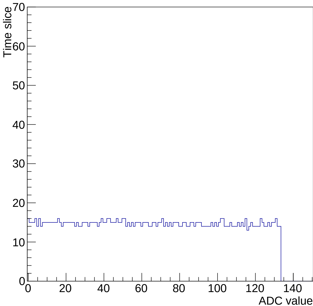
Evt 10 Time mcm 2000 chip 0 chan 6 34606-gain0-shaper7
