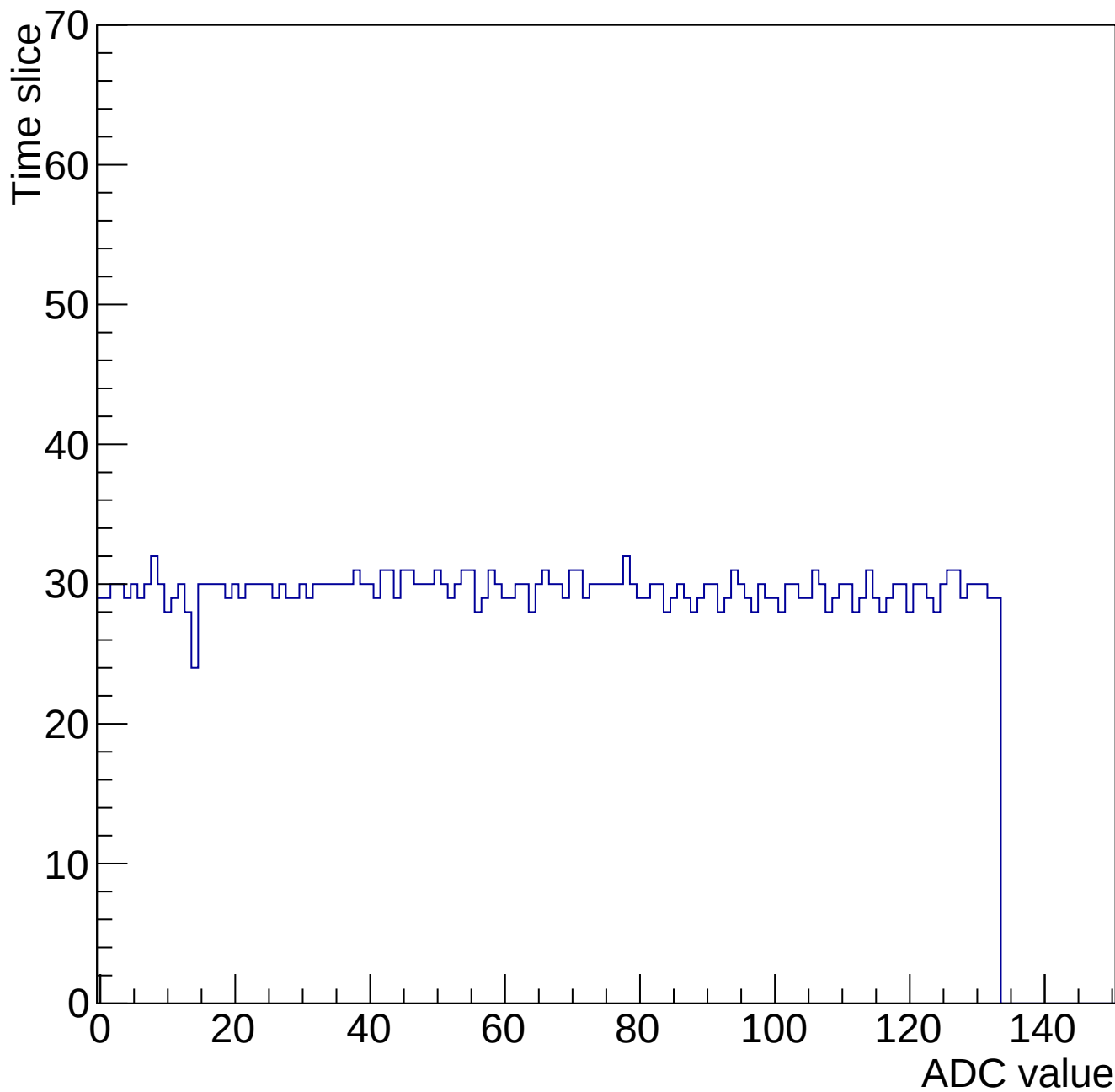
Evt 10 Time mcm 2000 chip 0 chan 1 34606-gain0-shaper7
