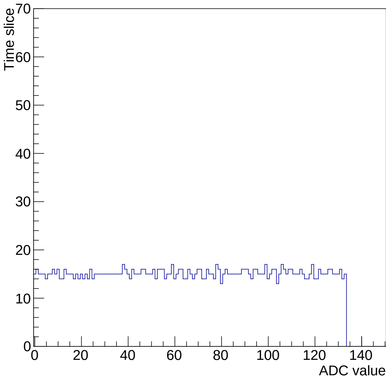
Evt 10 Time mcm 2000 chip 0 chan 0 34607-gain0-shaper7
