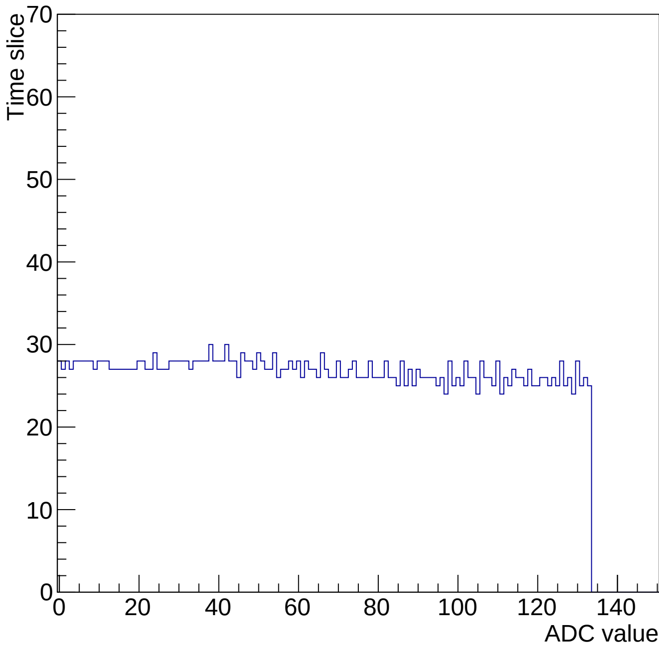
Evt 10 Time mcm 2000 chip 0 chan 5 34608-gain0-shaper7
