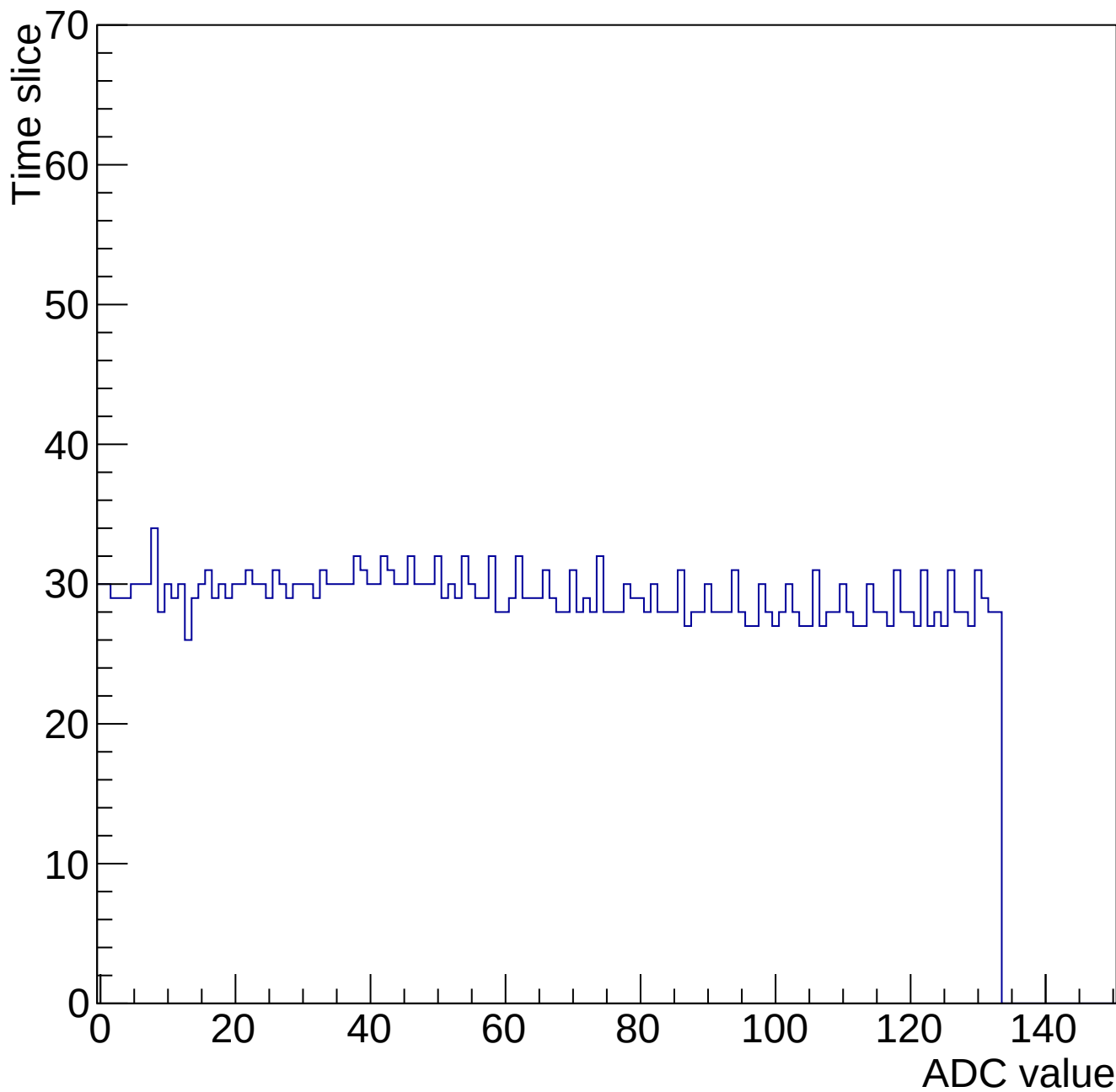
Evt 10 Time mcm 2000 chip 0 chan 1 34608-gain0-shaper7
