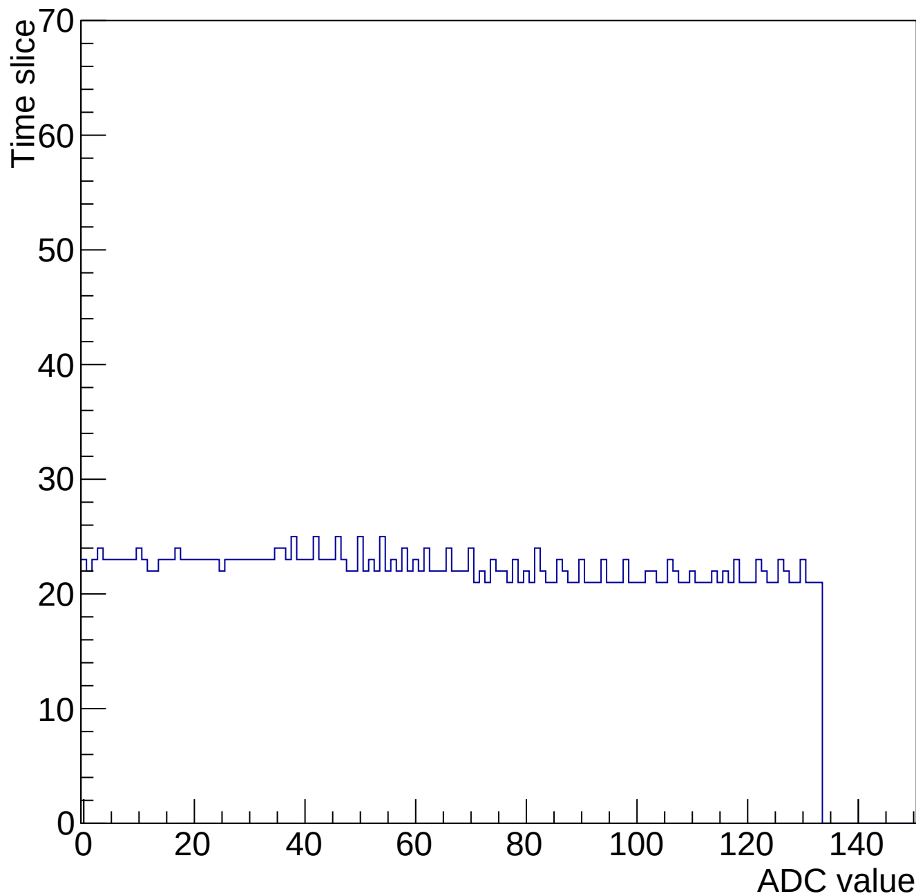
Evt 10 Time mcm 2000 chip 0 chan 7 34608-gain0-shaper7
