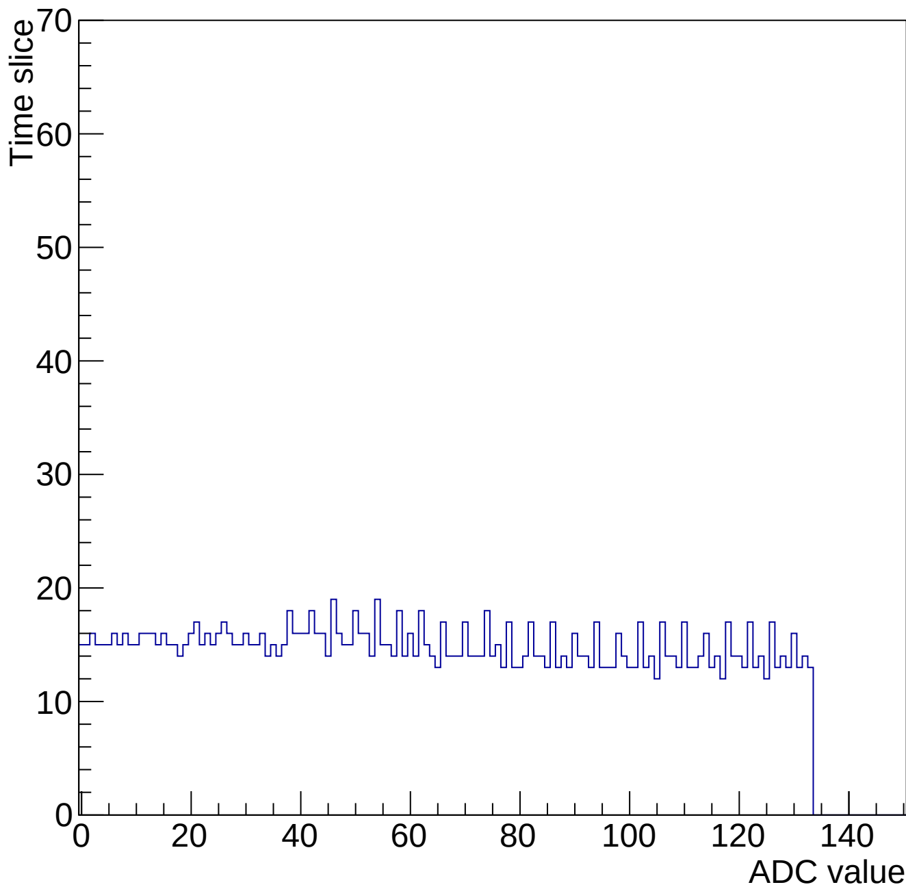
Evt 10 Time mcm 2000 chip 0 chan 0 34608-gain0-shaper7
