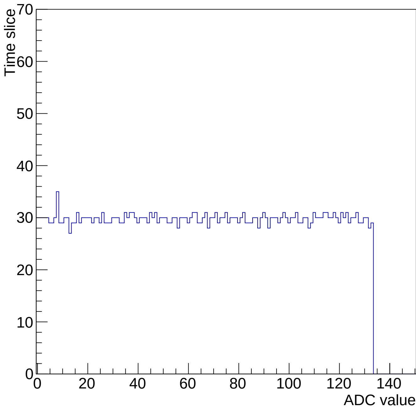
Evt 10 Time mcm 2000 chip 0 chan 1 34610-gain0-shaper7
