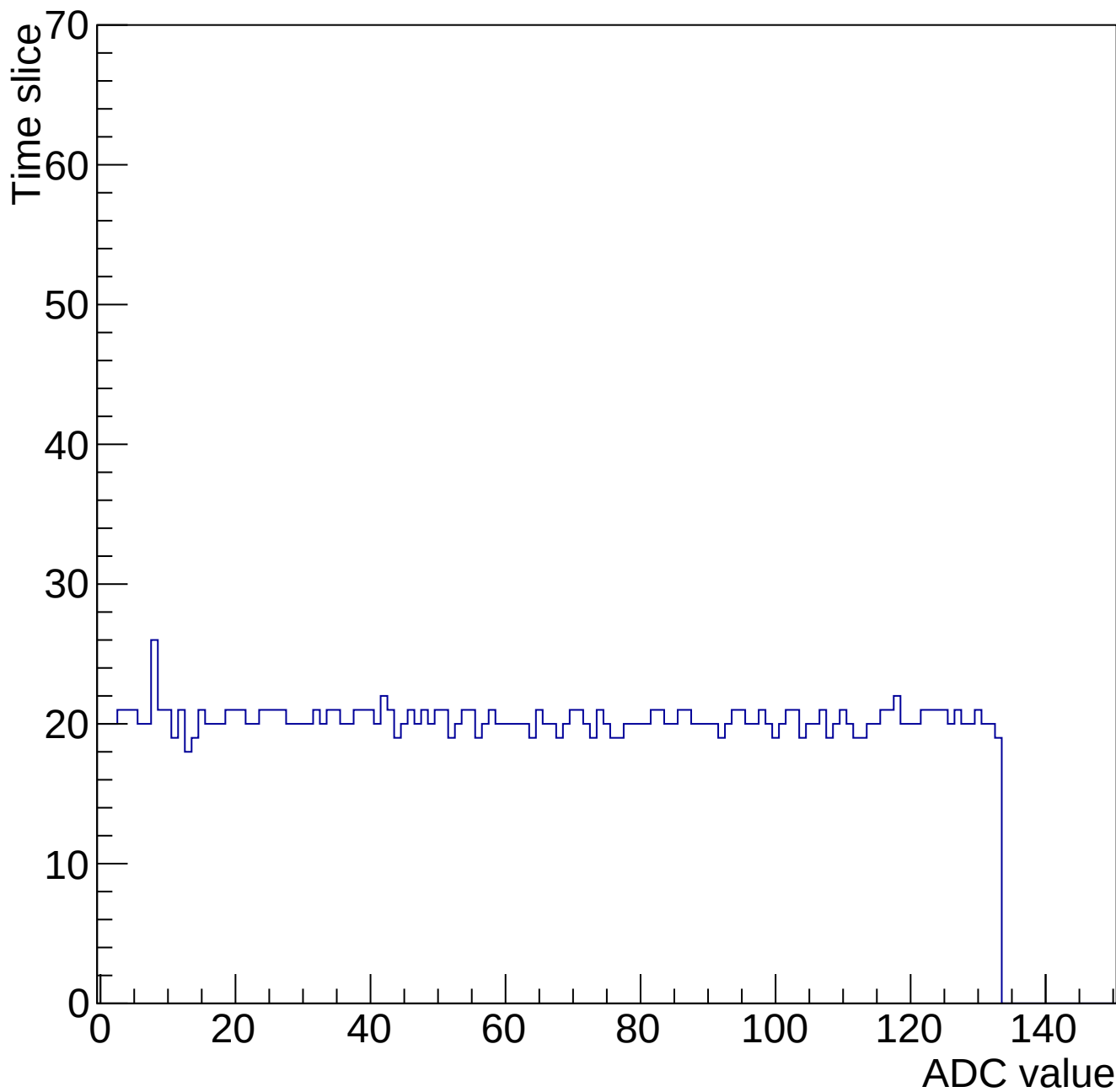
Evt 10 Time mcm 2000 chip 0 chan 2 34610-gain0-shaper7
