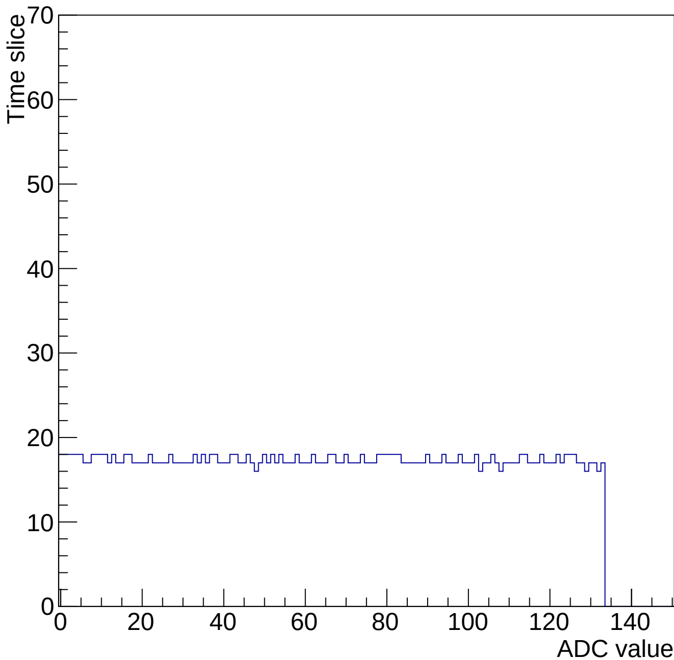
Evt 10 Time mcm 2000 chip 0 chan 9 34611-gain0-shaper7
