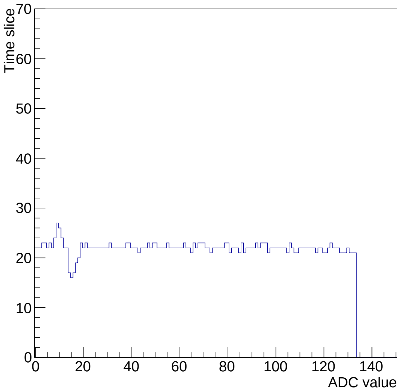
Evt 10 Time mcm 2000 chip 0 chan 2 34611-gain0-shaper7
