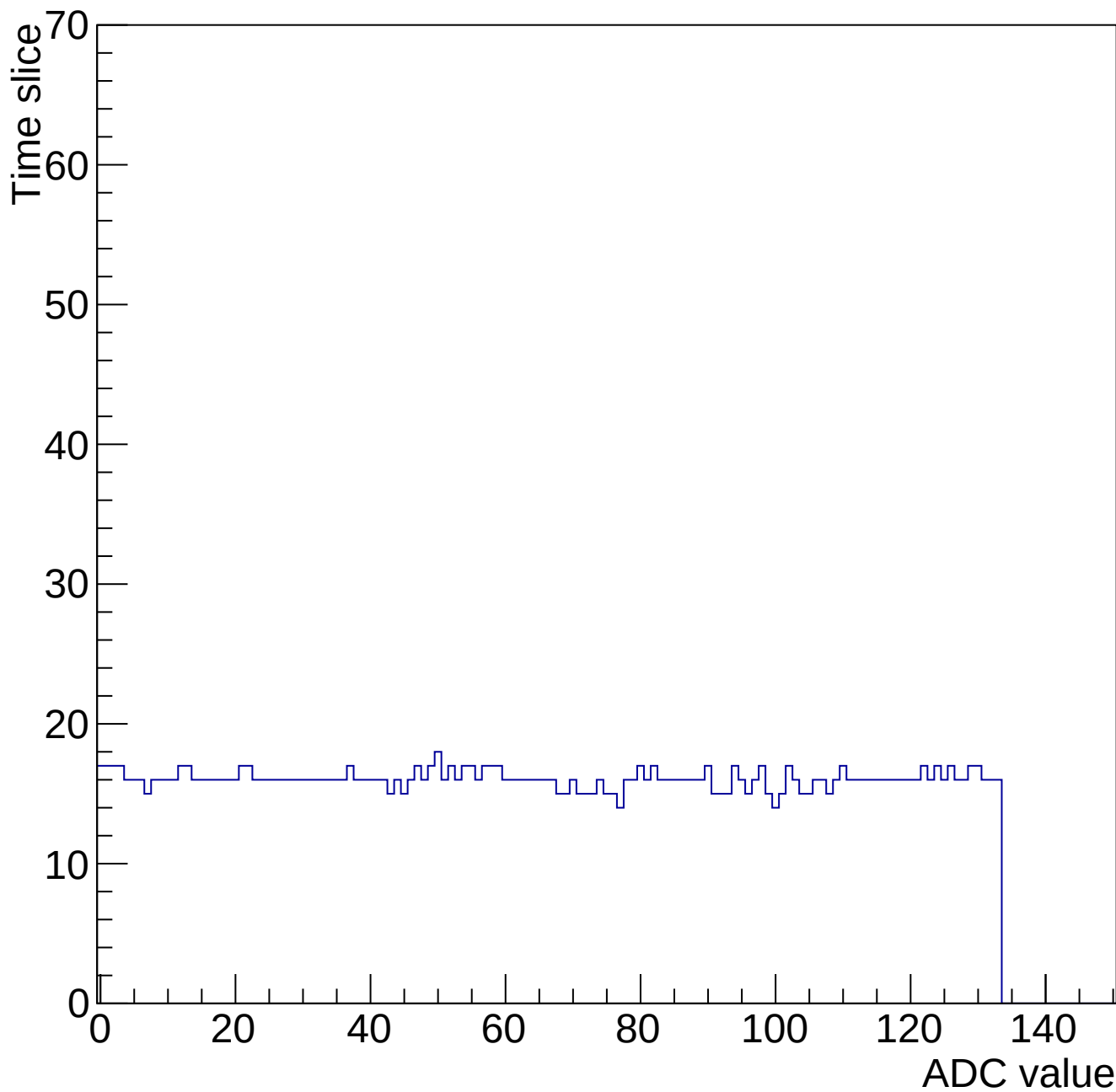
Evt 10 Time mcm 2000 chip 0 chan 6 34611-gain0-shaper7
