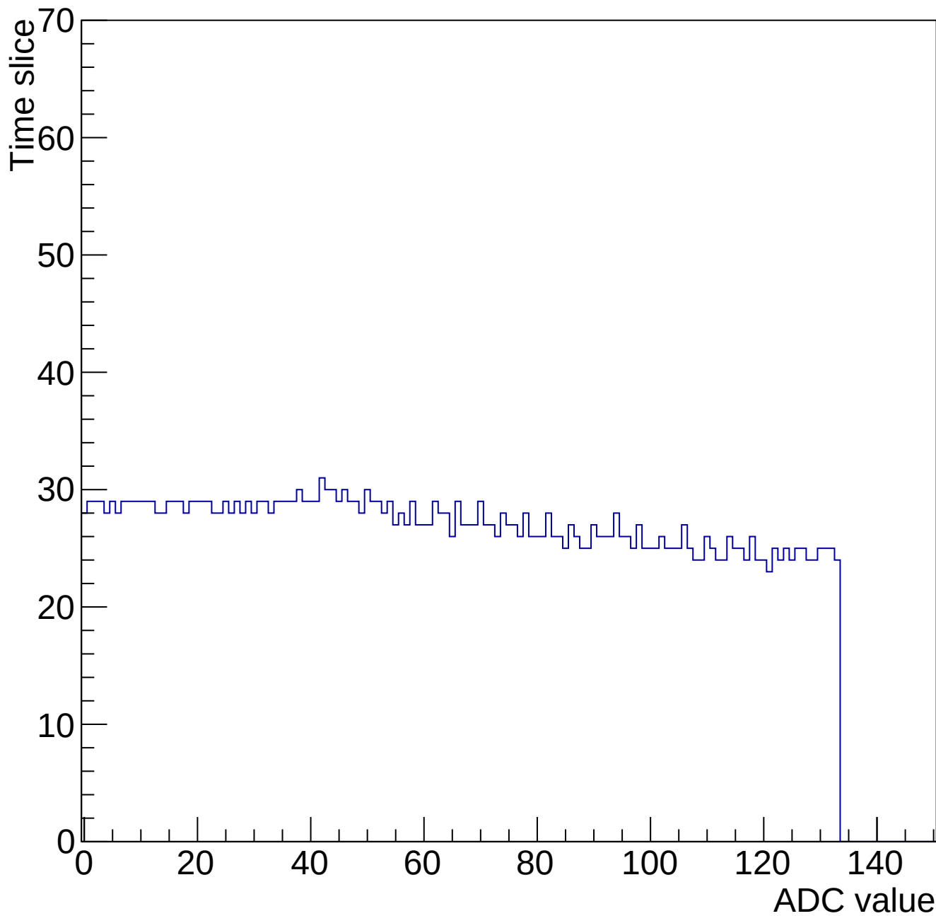
Evt 10 Time mcm 2000 chip 0 chan 8 34612-gain0-shaper0
