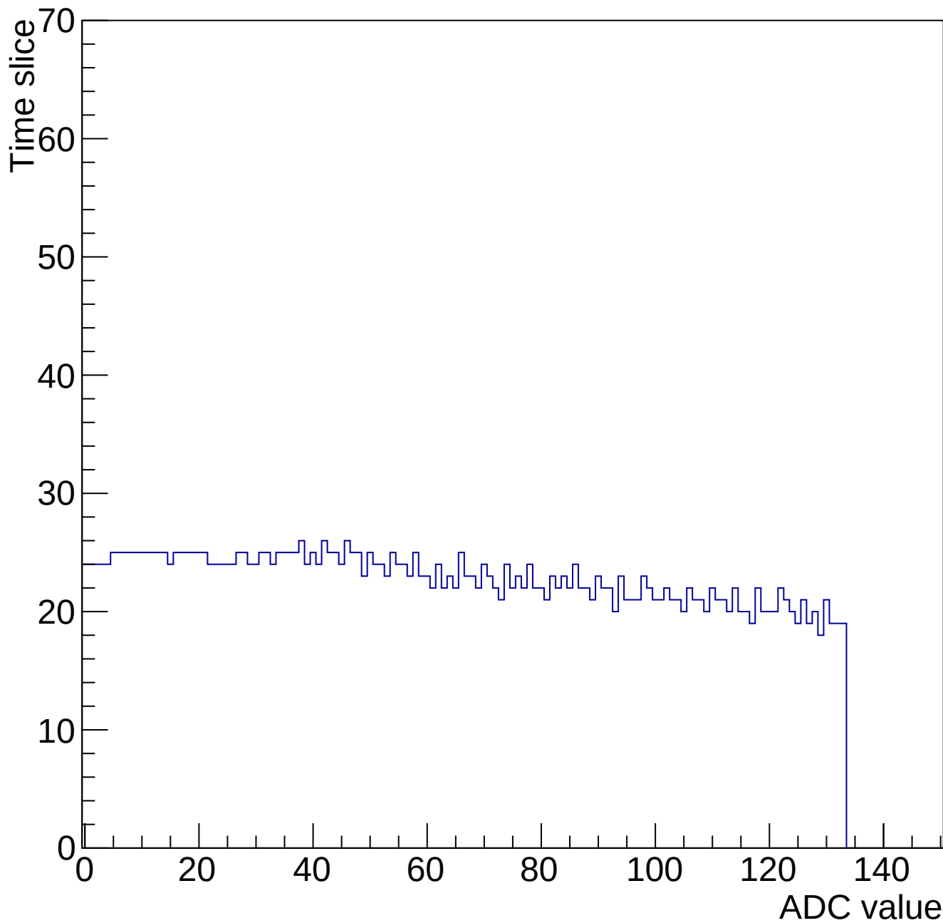
Evt 10 Time mcm 2000 chip 0 chan 4 34612-gain0-shaper0
