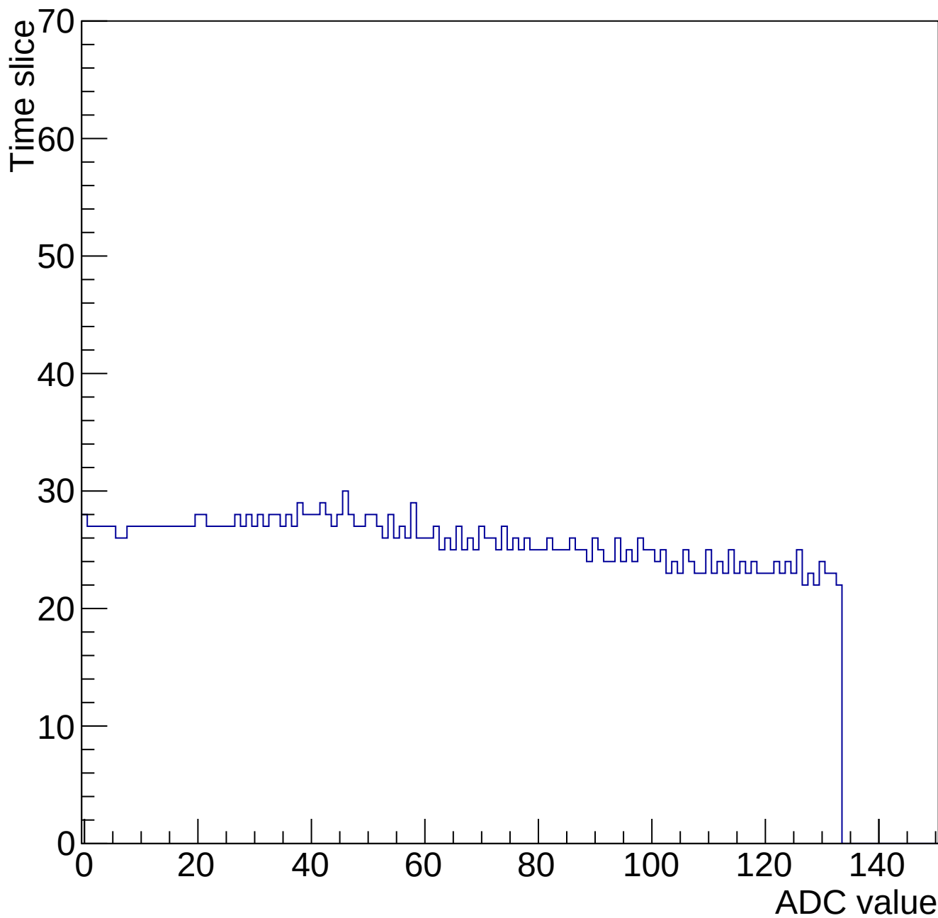
Evt 10 Time mcm 2000 chip 0 chan 7 34612-gain0-shaper0
