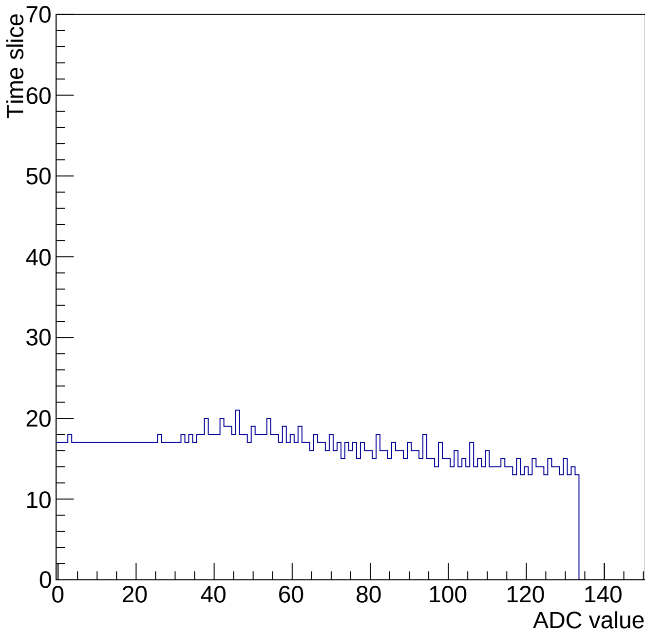
Evt 10 Time mcm 2000 chip 0 chan 9 34612-gain0-shaper0
