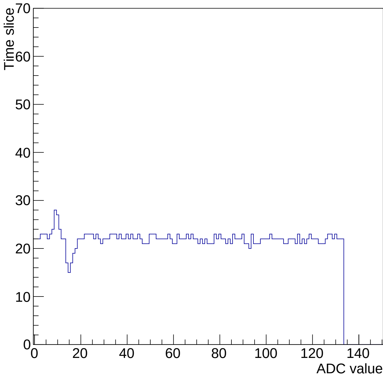
Evt 10 Time mcm 2000 chip 0 chan 2 34614-gain0-shaper0
