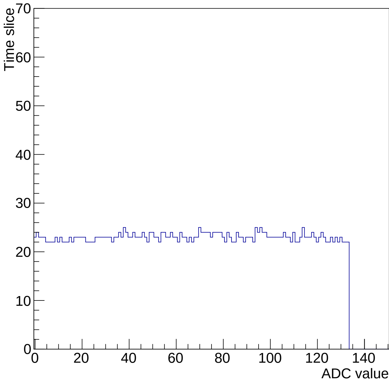
Evt 10 Time mcm 2000 chip 0 chan 3 34614-gain0-shaper0
