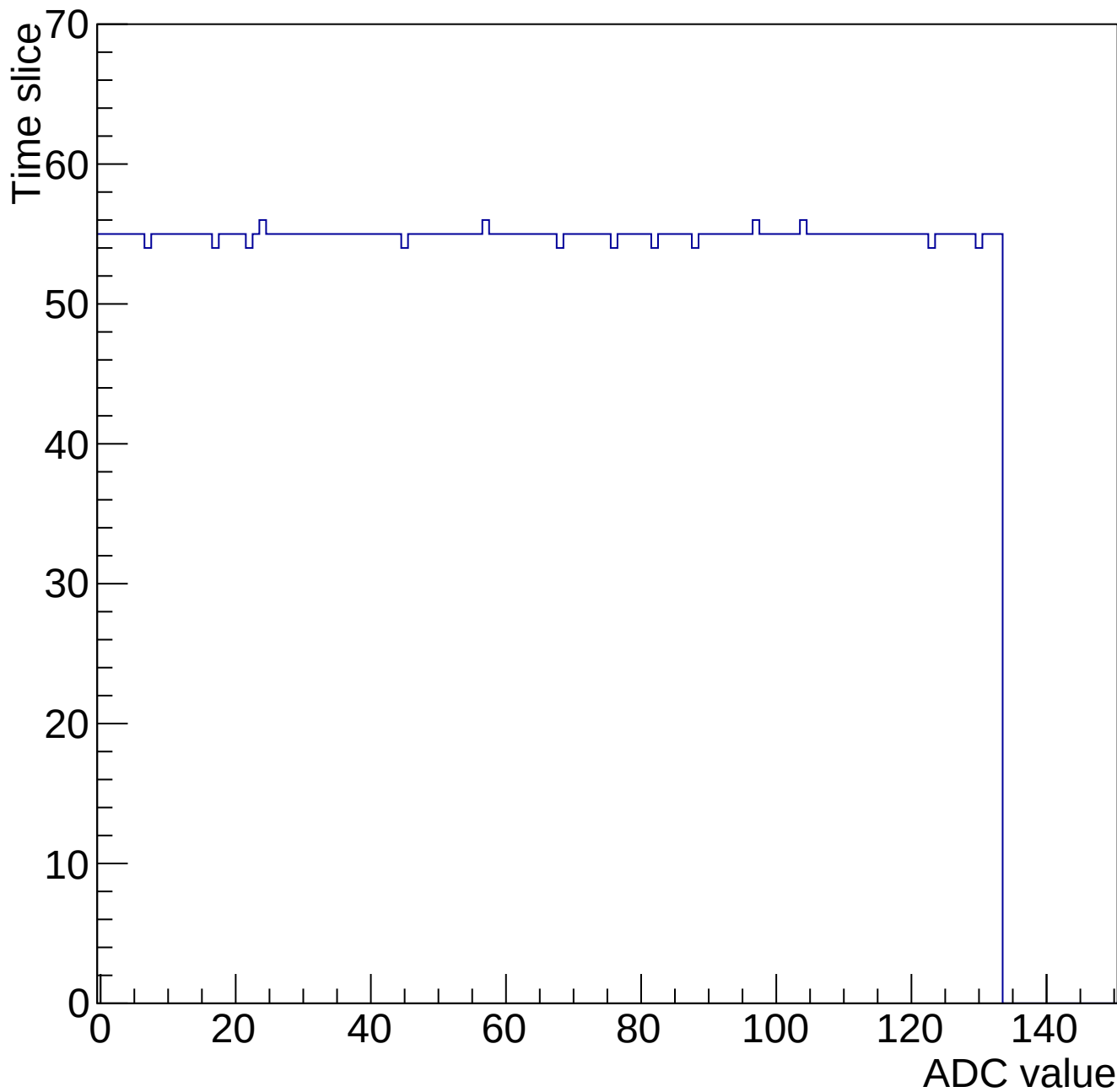
Evt 10 Time mcm 2000 chip 0 chan 8 gain0-shaper4
