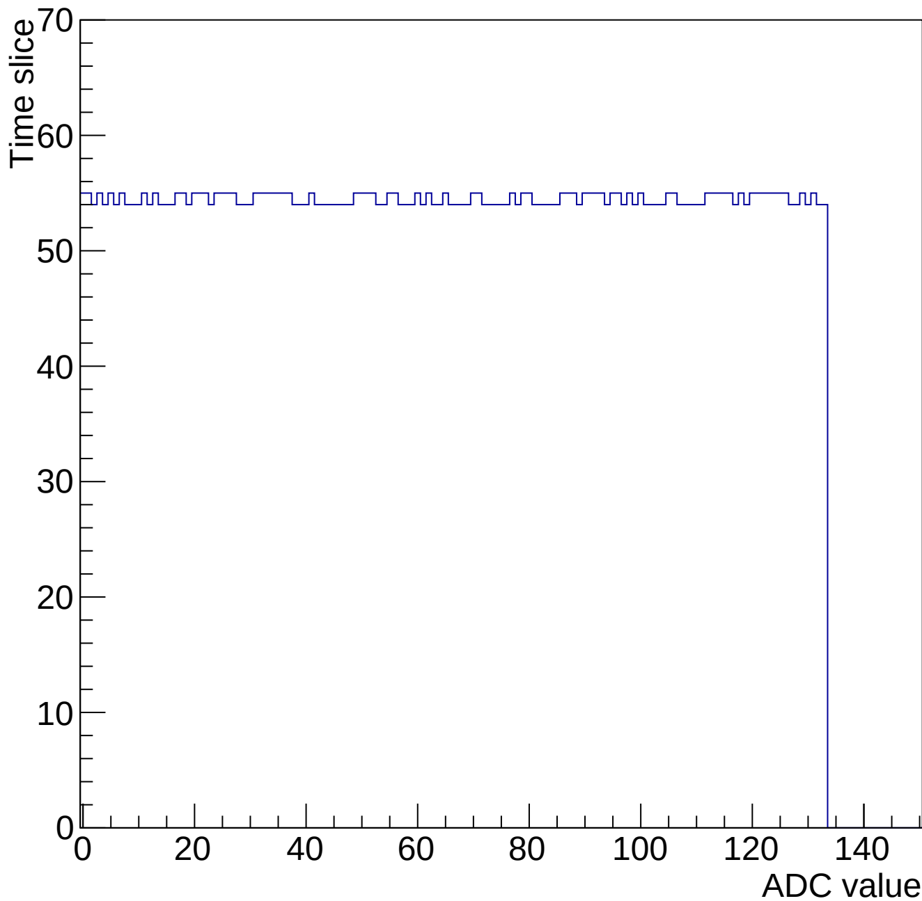
Evt 10 Time mcm 2000 chip 0 chan 7 gain0-shaper4
