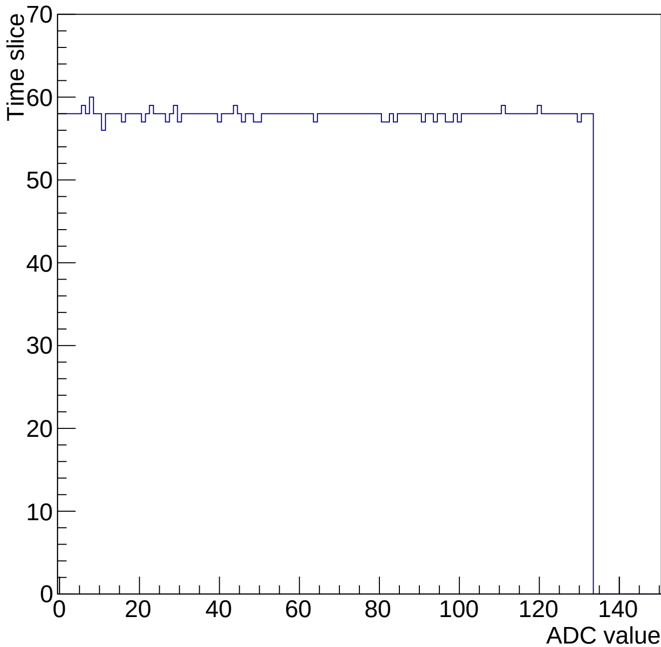
Evt 10 Time mcm 2000 chip 0 chan 1 gain0-shaper4
