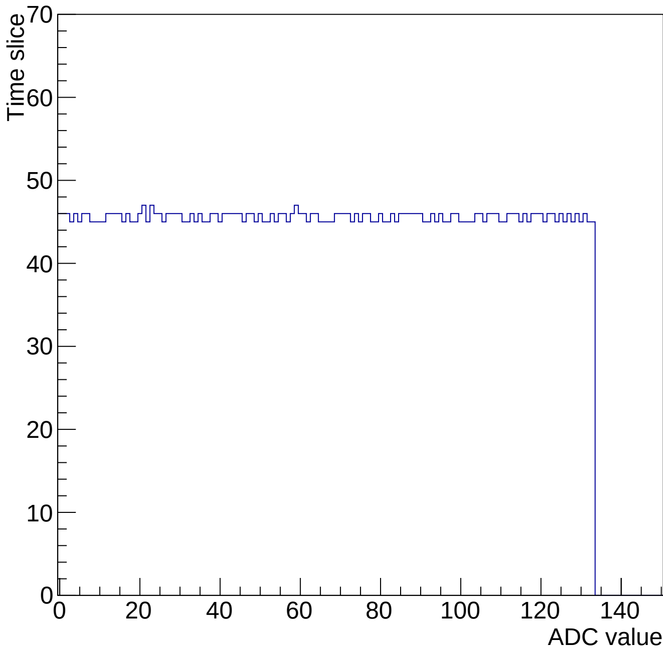
Evt 10 Time mcm 2000 chip 0 chan 0 gain0-shaper6
