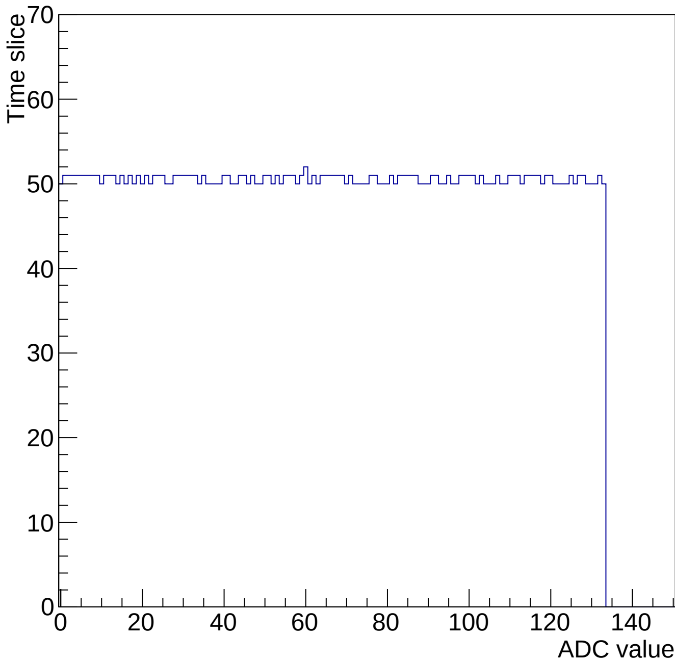
Evt 10 Time mcm 2000 chip 0 chan 4 gain0-shaper6
