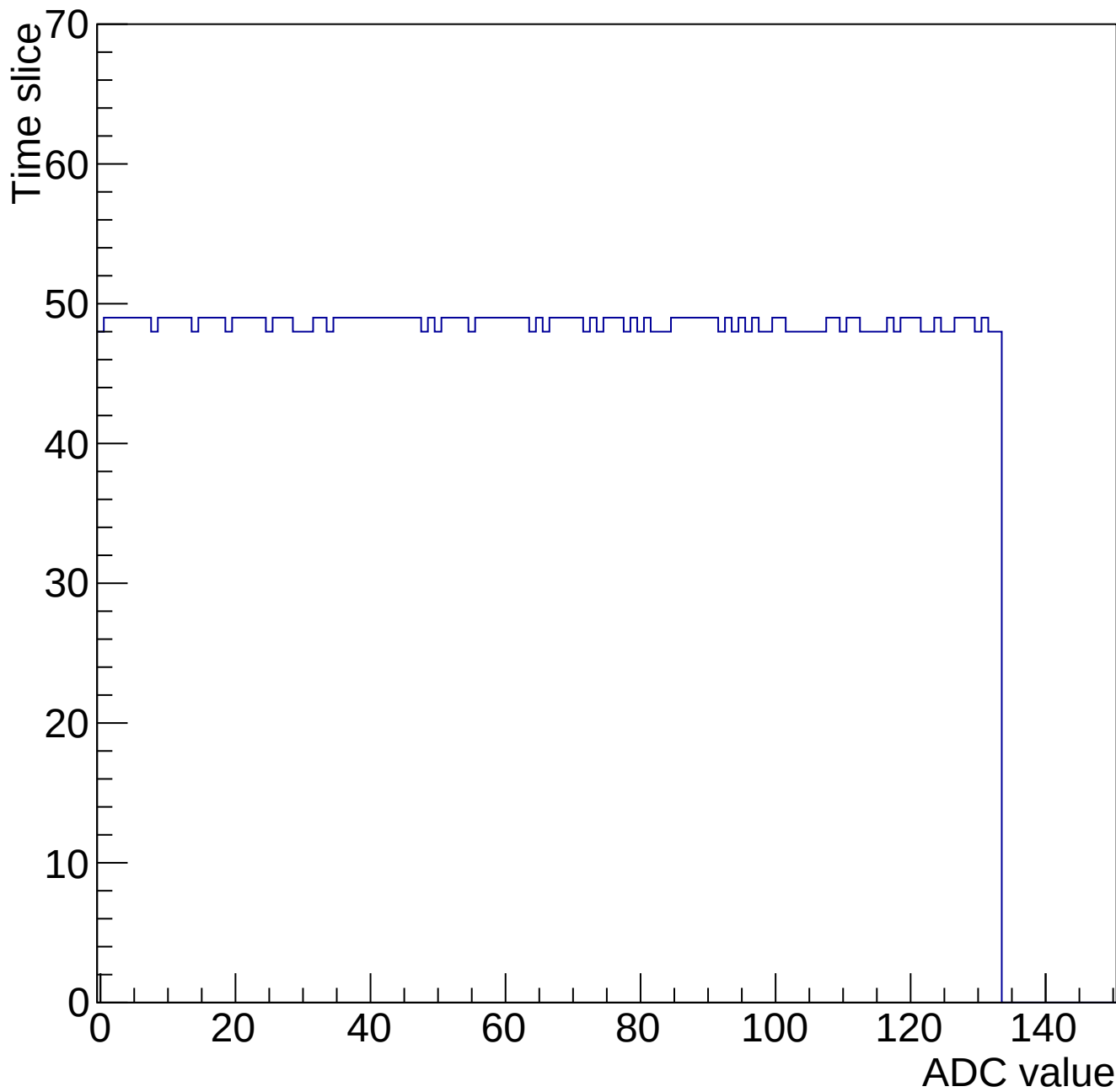
Evt 10 Time mcm 2000 chip 0 chan 15 gain0-shaper6
