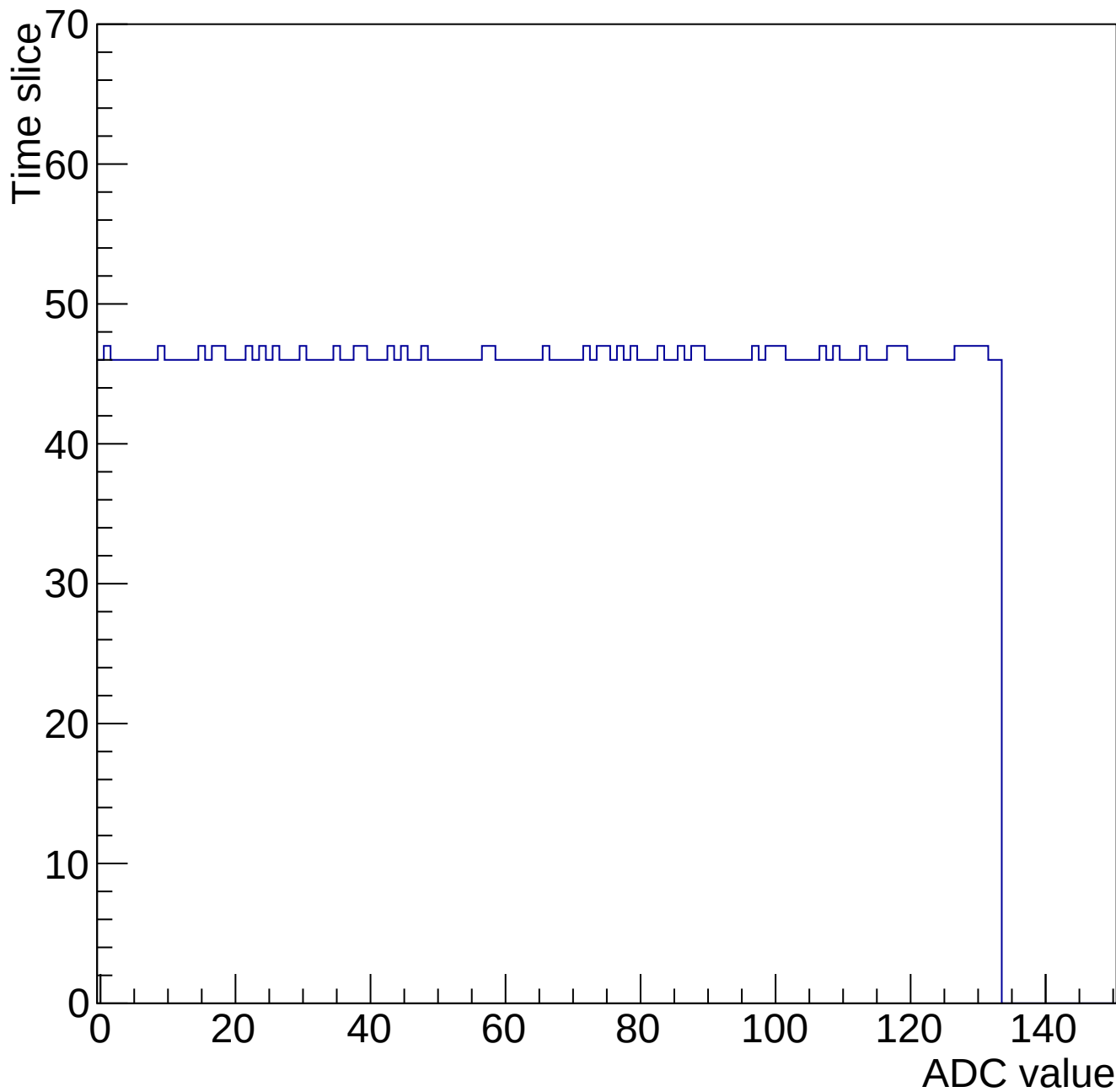
Evt 10 Time mcm 2000 chip 0 chan 6 gain0-shaper6
