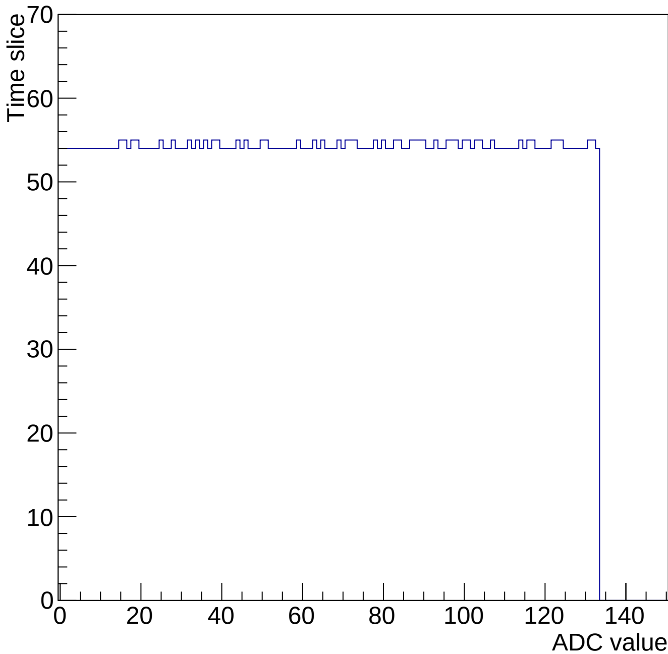
Evt 10 Time mcm 2000 chip 0 chan 7 gain0-shaper6
