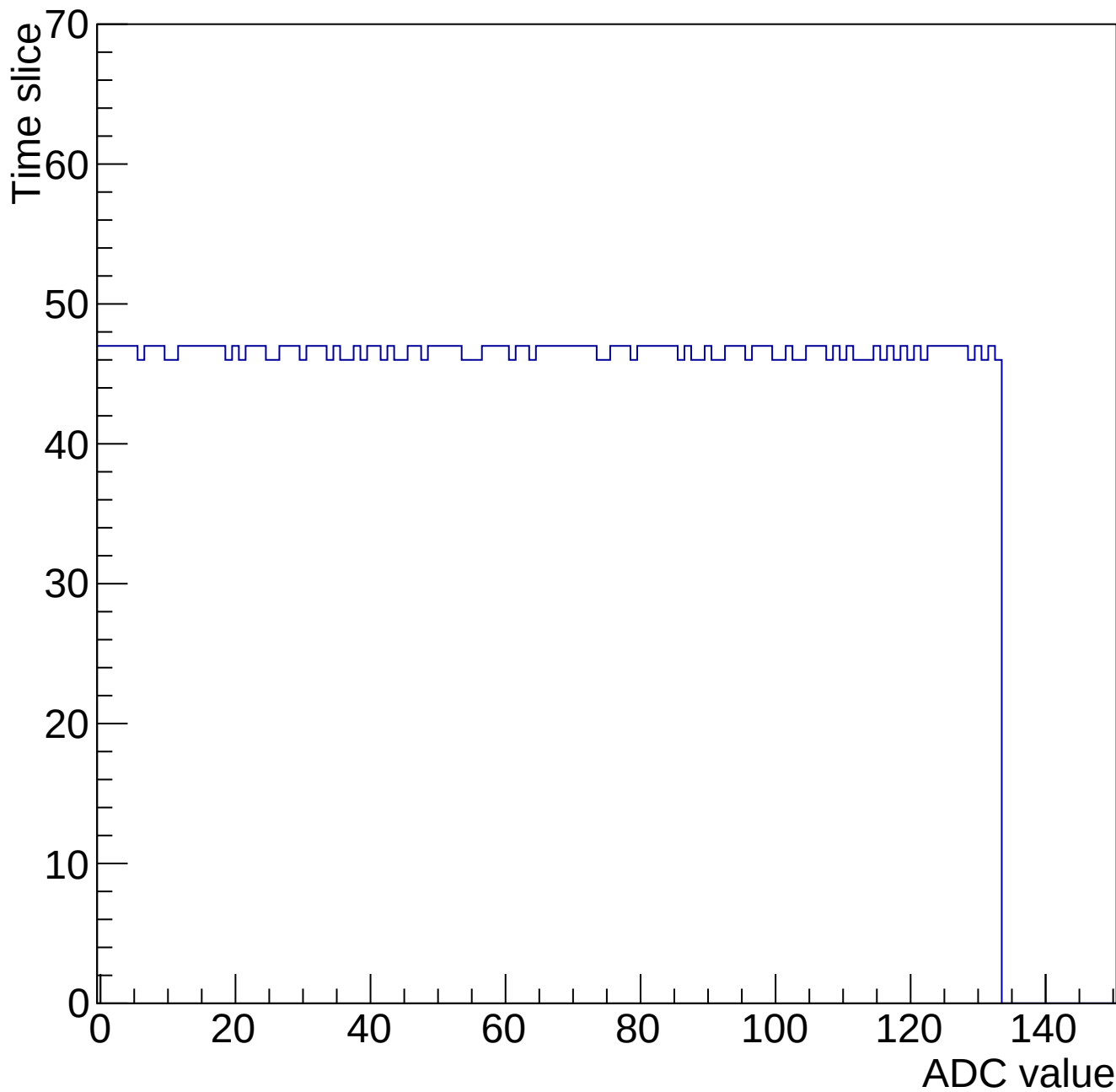
Evt 10 Time mcm 2000 chip 0 chan 10 gain0-shaper6
