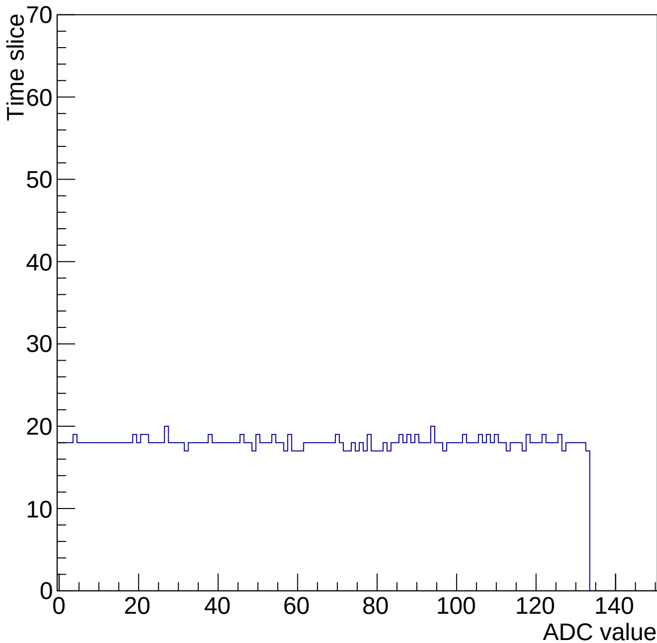
Evt 20 Time mcm 2000 chip 0 chan 0 34603-gain0-shaper0
