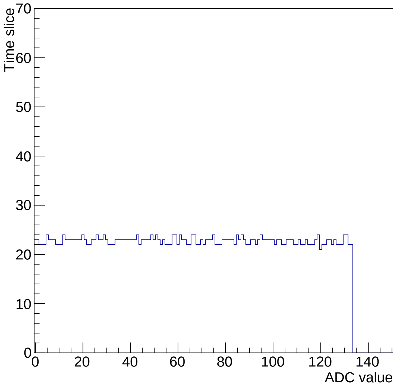
Evt 20 Time mcm 2000 chip 0 chan 7 34604-gain0-shaper7
