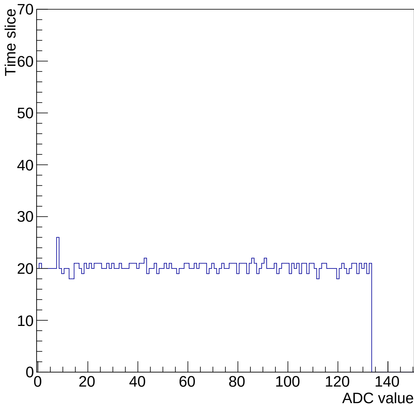
Evt 20 Time mcm 2000 chip 0 chan 2 34604-gain0-shaper7
