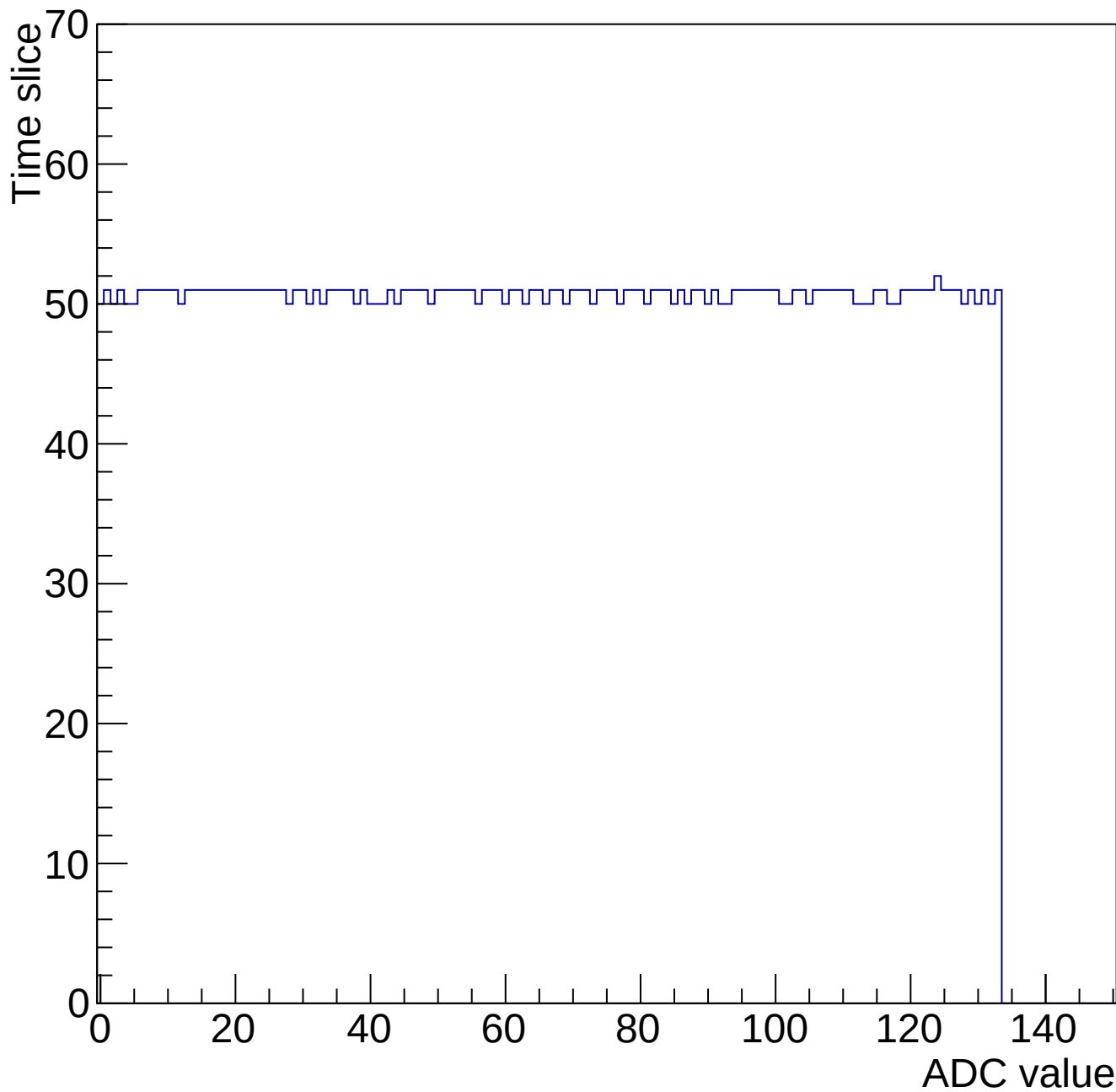
Evt 20 Time mcm 2000 chip 0 chan 4 gain0-shaper6
