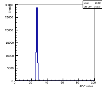
Pedestals ch 7 chip 2000 gain0-shaper0
