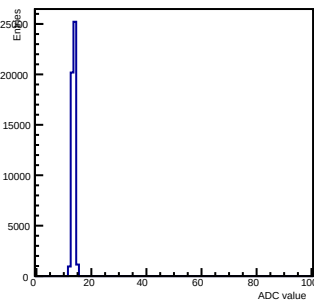
Pedestals ch 12 chip 2007 gain0-shaper0
