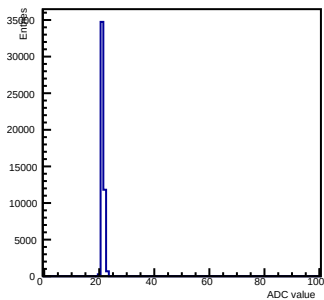
Pedestals ch 11 chip 2007 gain0-shaper0
