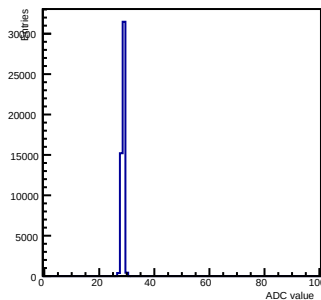
Pedestals ch 14 chip 2007 gain0-shaper0
