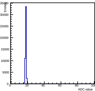
Pedestals ch 8 chip 2007 gain0-shaper0
