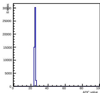
Pedestals ch 6 chip 2007 gain0-shaper0
