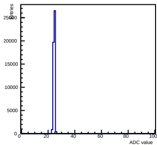
Pedestals ch 1 chip 2007 gain0-shaper0
