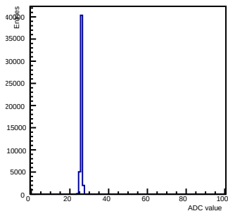
Pedestals ch 13 chip 2007 gain0-shaper0
