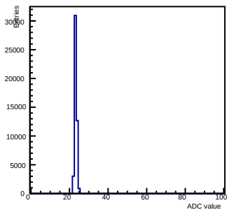
Pedestals ch 3 chip 2007 gain0-shaper0
