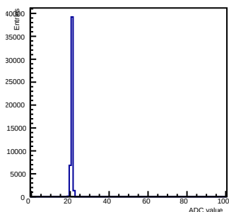
Pedestals ch 5 chip 2007 gain0-shaper0
