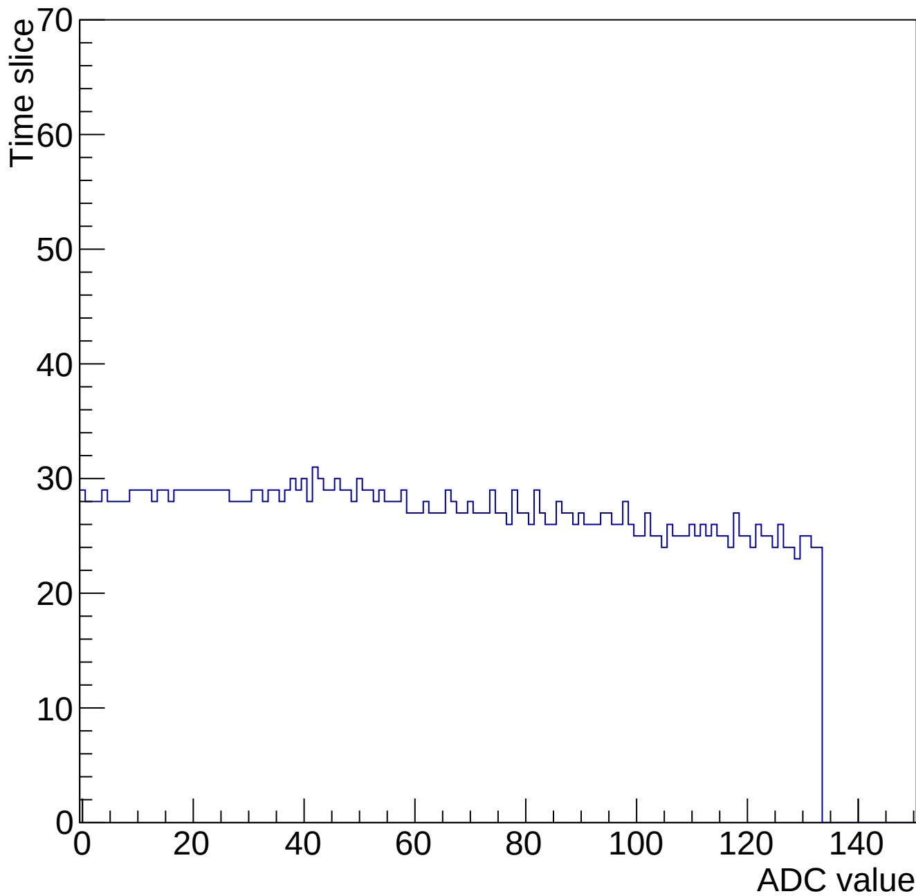
Evt 10 Time mcm 2000 chip 0 chan 12 34618-gain0-shaper0
