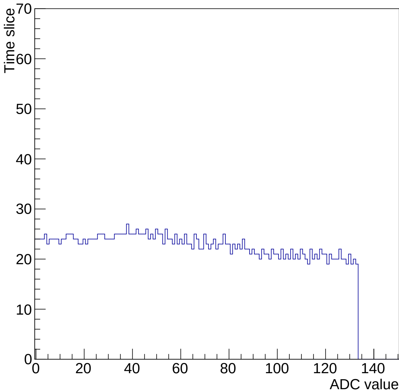
Evt 10 Time mcm 2000 chip 0 chan 4 34618-gain0-shaper0
