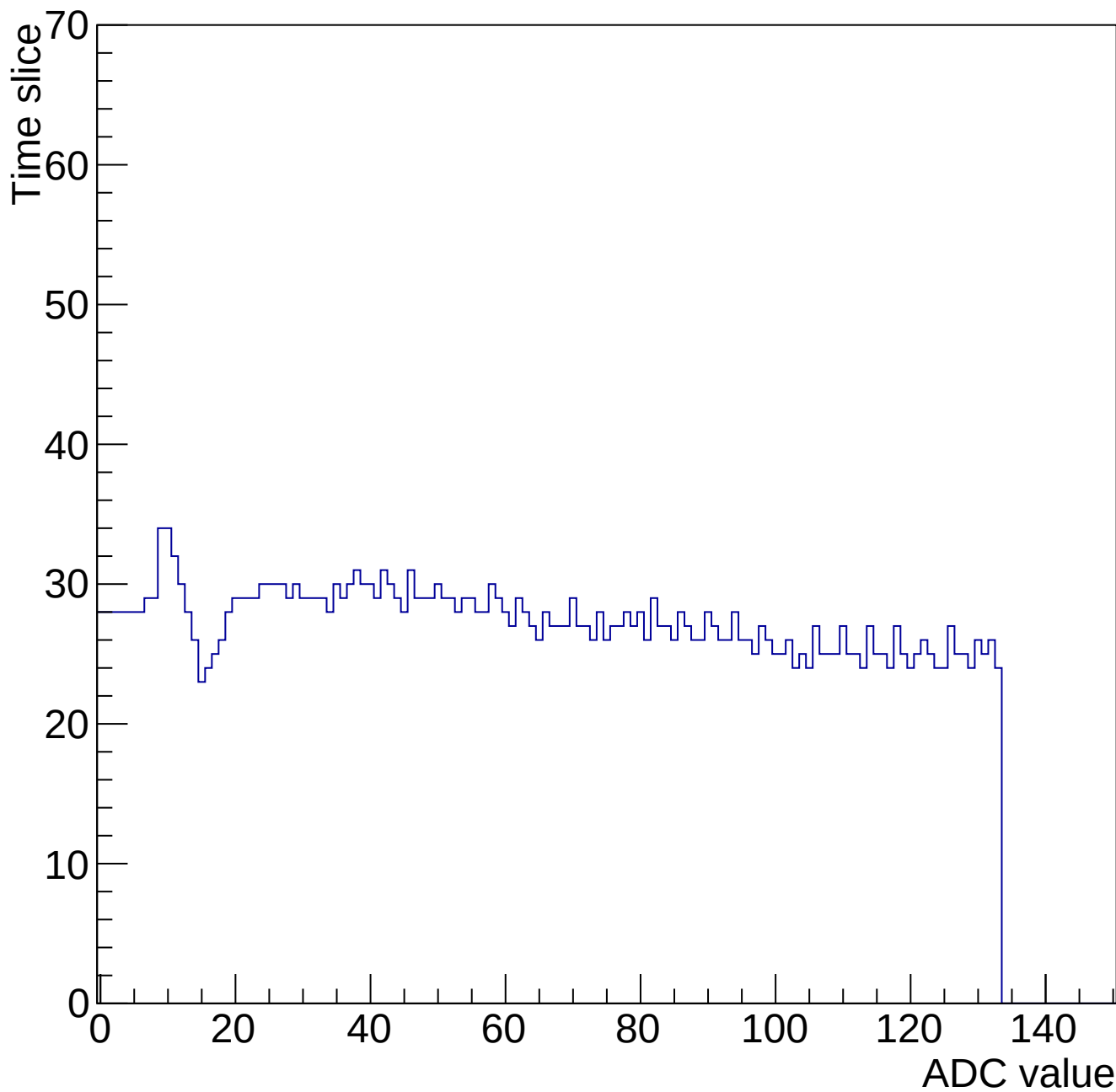
Evt 10 Time mcm 2000 chip 0 chan 1 34618-gain0-shaper0
