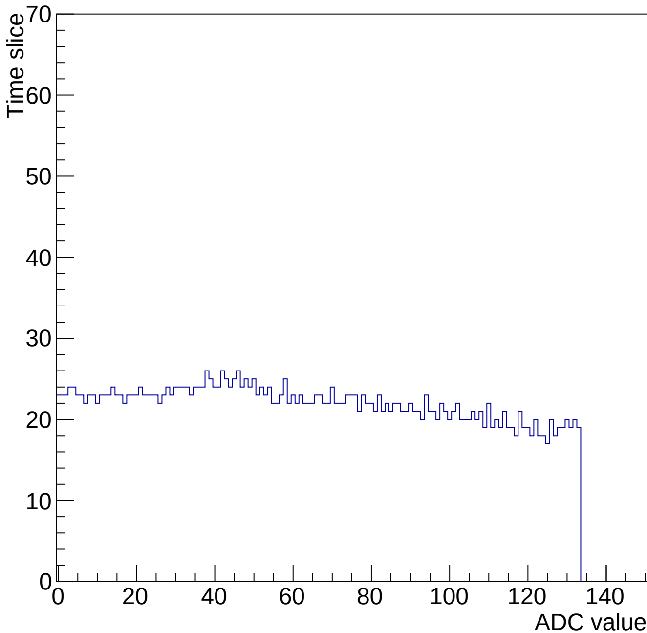
Evt 10 Time mcm 2000 chip 0 chan 3 34618-gain0-shaper0
