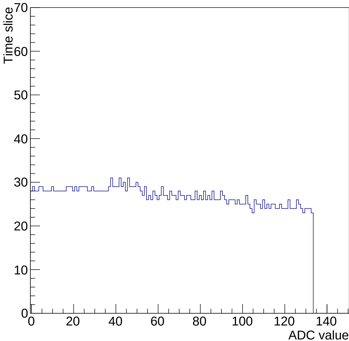
Evt 10 Time mcm 2000 chip 0 chan 8 34618-gain0-shaper0
