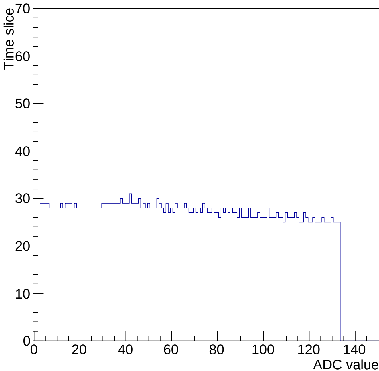
Evt 10 Time mcm 2000 chip 0 chan 8 34621-gain0-shaper0
