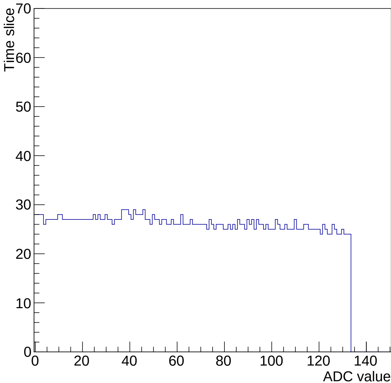
Evt 10 Time mcm 2000 chip 0 chan 7 34622-gain0-shaper0
