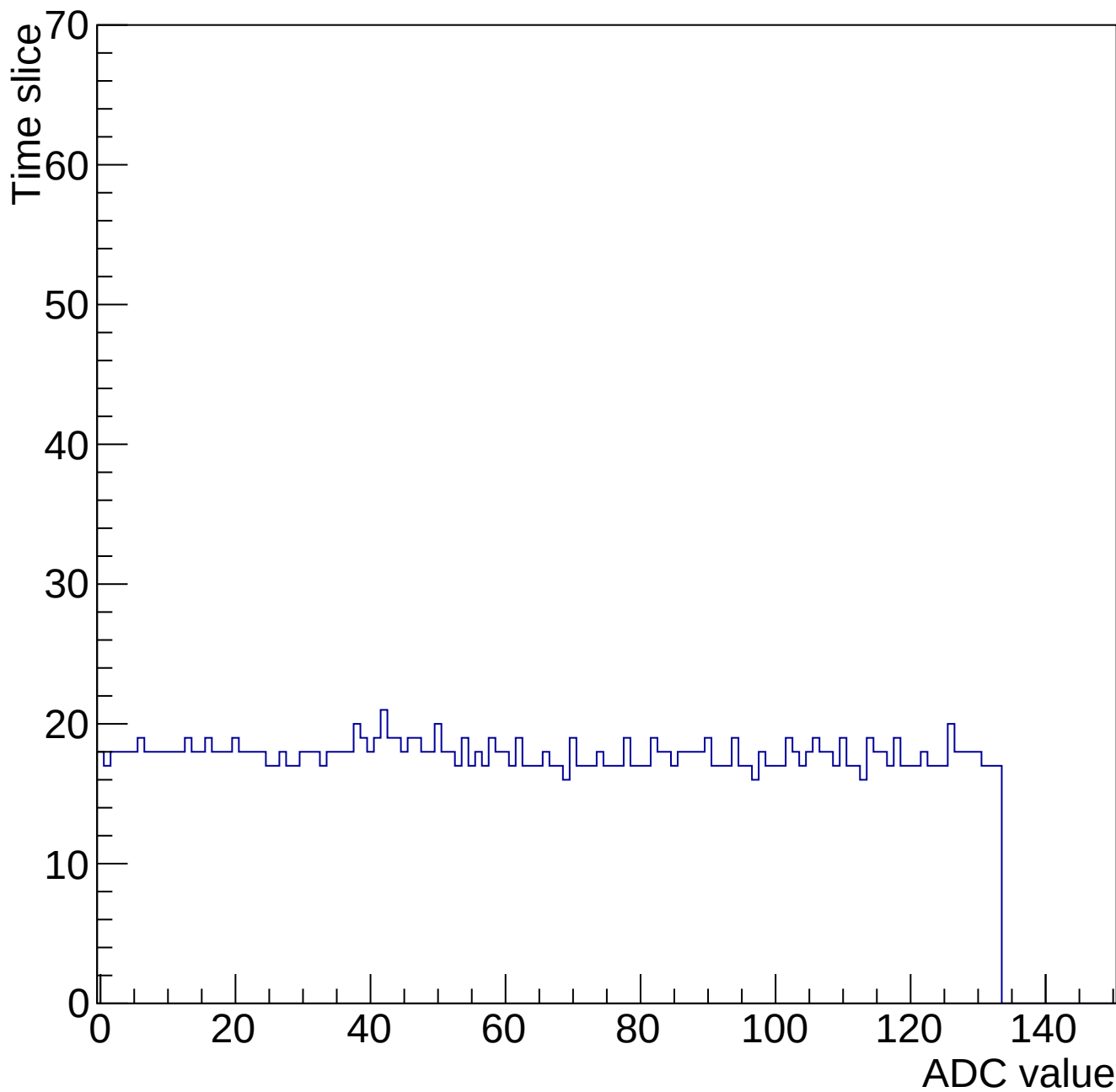
Evt 10 Time mcm 2000 chip 0 chan 0 34623-gain0-shaper0
